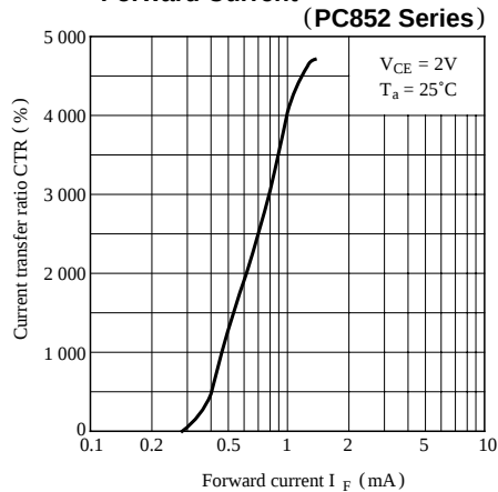
Fig. 5-a Current Transfer Ratio vs. Forward Current
