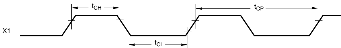
FIGURE 14-2. Clock Timing
