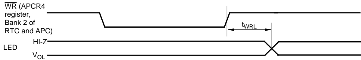
FIGURE 14-38. LED Timing
