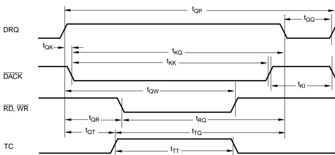
FIGURE 14-14. FDC DMA Timing
