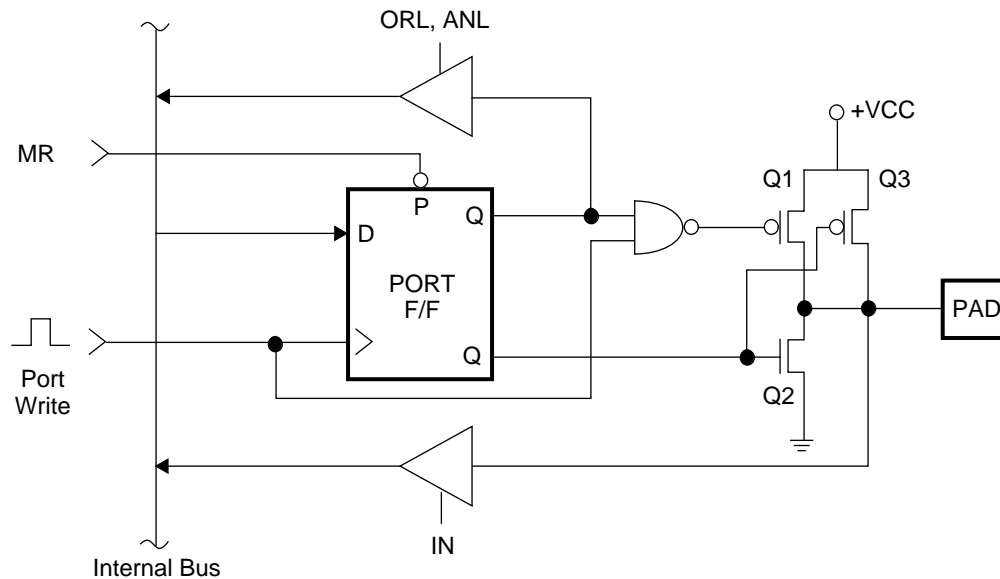
FIGURE 3-6. Quasi-Bidirectional Driver
