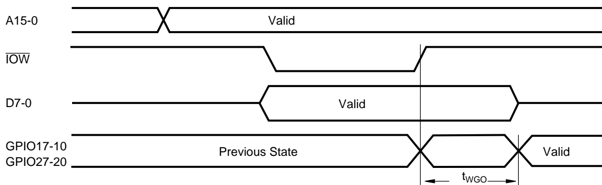
FIGURE 14-28. GPIO Write Timing Diagram
