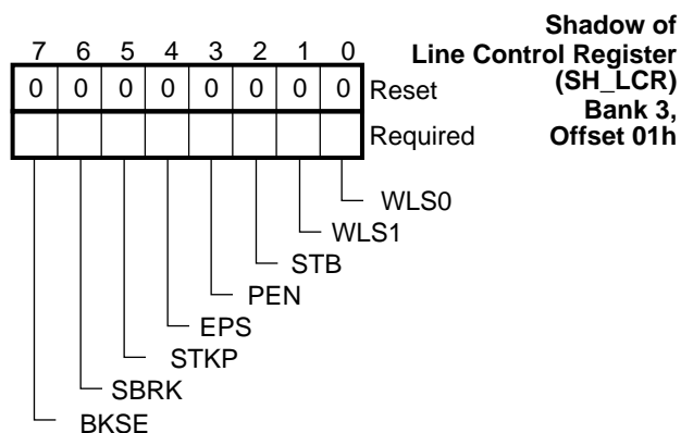
FIGURE 8-27. SH_LCR Register Bitmap
