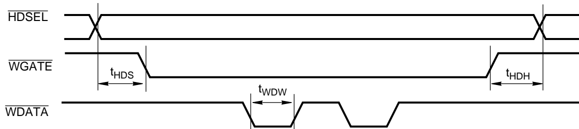
FIGURE 14-18. Write Data Timing
