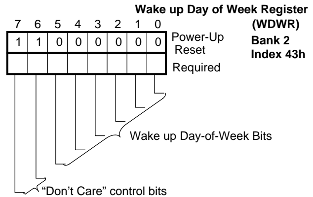
FIGURE 4-17. WDWR Register Bitmap
