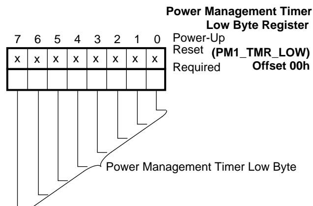
FIGURE 4-38. PM1_TMR_LOW Register Bitmap
