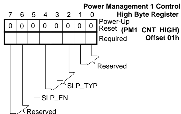
FIGURE 4-37. PM1_CNT_HIGH Register Bitmap
