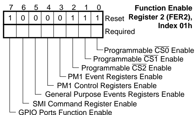
FIGURE 10-4. FER2 Register Bitmap
