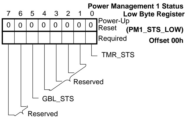
FIGURE 4-32. PM1_STS_LOW Register Bitmap
