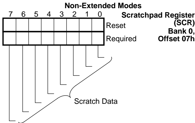
FIGURE 7-17. SPR Register Bitmap
