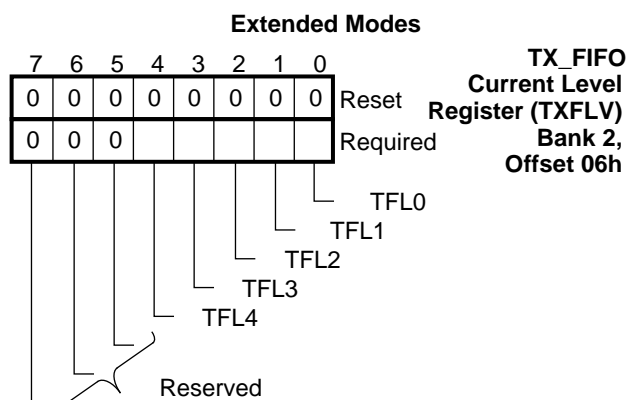
FIGURE 8-24. TXFLV Register Bitmap
