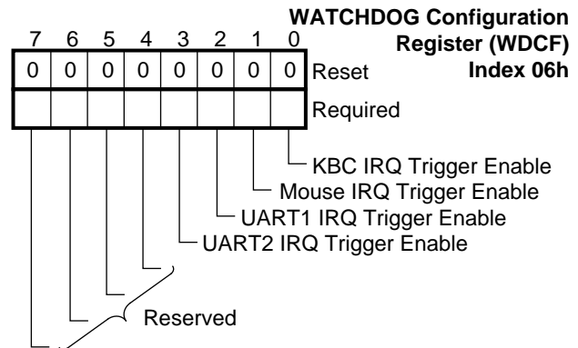
FIGURE 10-9. WDCF Register Bitmap
