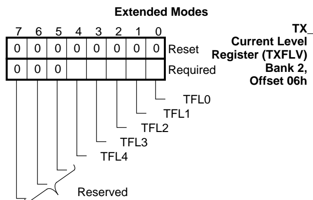
FIGURE 7-26. TXFLV Register Bitmap
