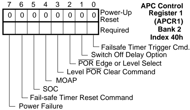
FIGURE 4-14. APCR1 Register Bitmap
