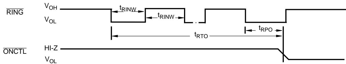
FIGURE 14-34. \overline{\text{RING}} Trigger and \overline{\text{ONCTL}} Timing
