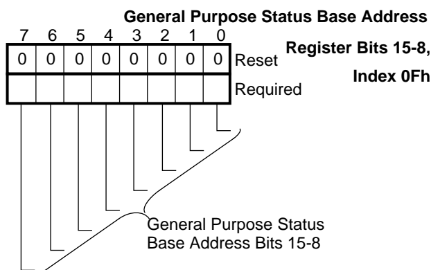
FIGURE 10-18. General Purpose Base Address Bits 15-8 Register Bitmap
