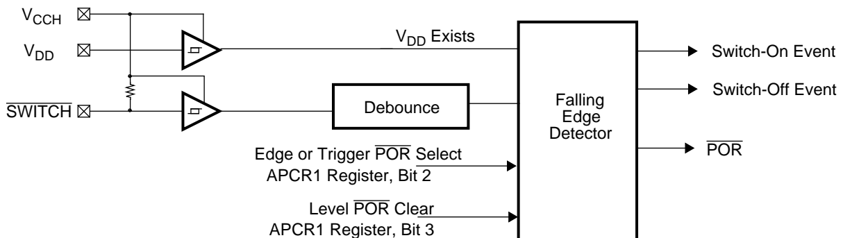
FIGURE 4-13. Switch Event Detector
