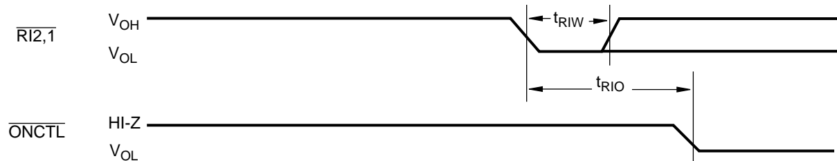
FIGURE 14-33. \overline{\text{RI}} Trigger and \overline{\text{ONCTL}} Timing
