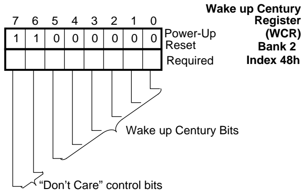
FIGURE 4-22. WCR Register Bitmap
