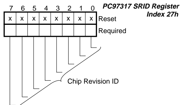
FIGURE 2-8. PC97317 SRID Register Bitmap
