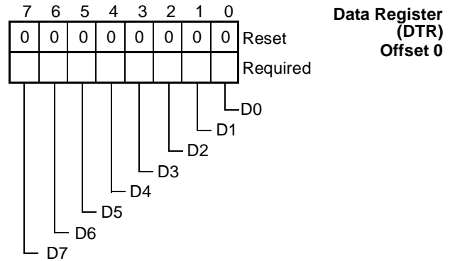
FIGURE 60. DTR Register Bitmap (SPP Mode)
