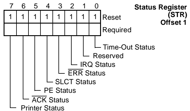
FIGURE 61. STR Register Bitmap (SPP Mode)
