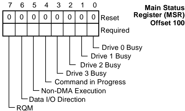
FIGURE 49. MSR Register Bitmap
