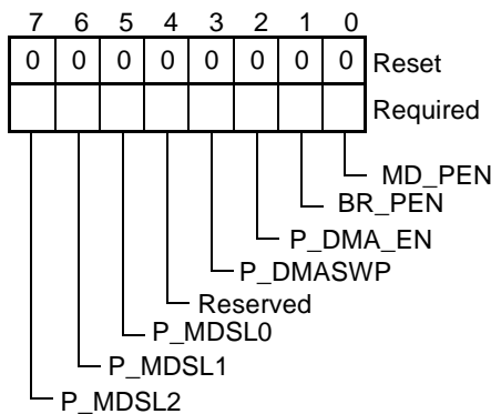
FIGURE 88. Pipelined Mode Register
