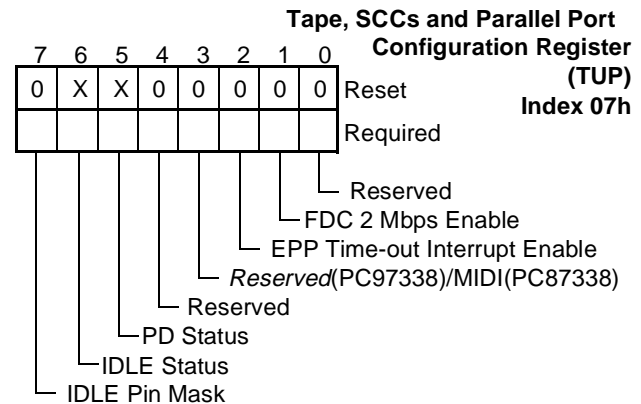
FIGURE 9. TUP Register Bitmap
