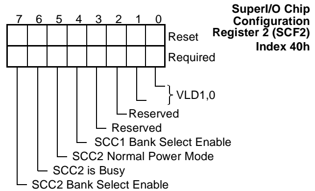
FIGURE 22. SCF2 Register Bitmap
