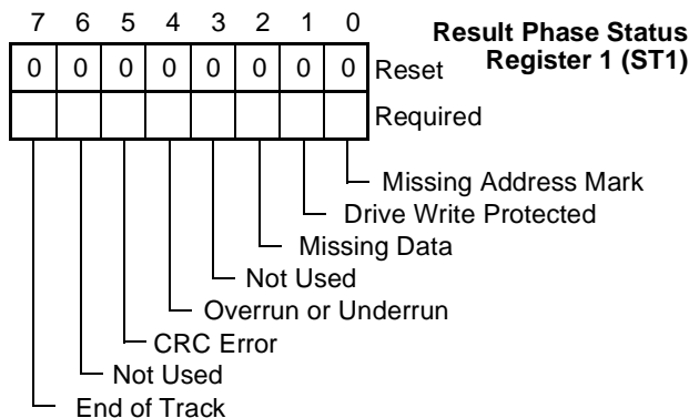
FIGURE 55. ST1 Result Phase Register Bitmap
