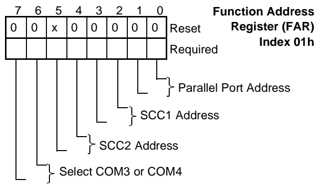
FIGURE 4. FAR Register Bitmap
