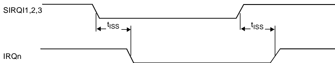
FIGURE 109. System Interrupts Timing
