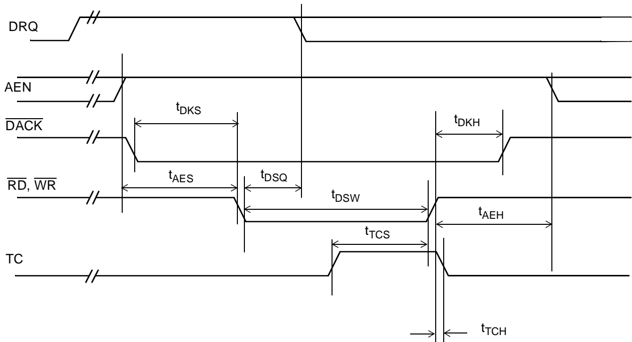
FIGURE 94. DMA Access Timing
