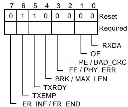
FIGURE 88. Link Status Register
