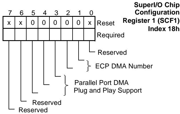
FIGURE 19. SCF1 Register Bitmap
