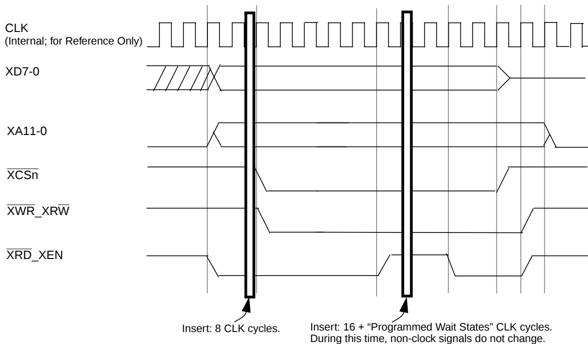
Figure 22. Mode 1, Normal Address X-Bus Transaction - Write Access Cycle
