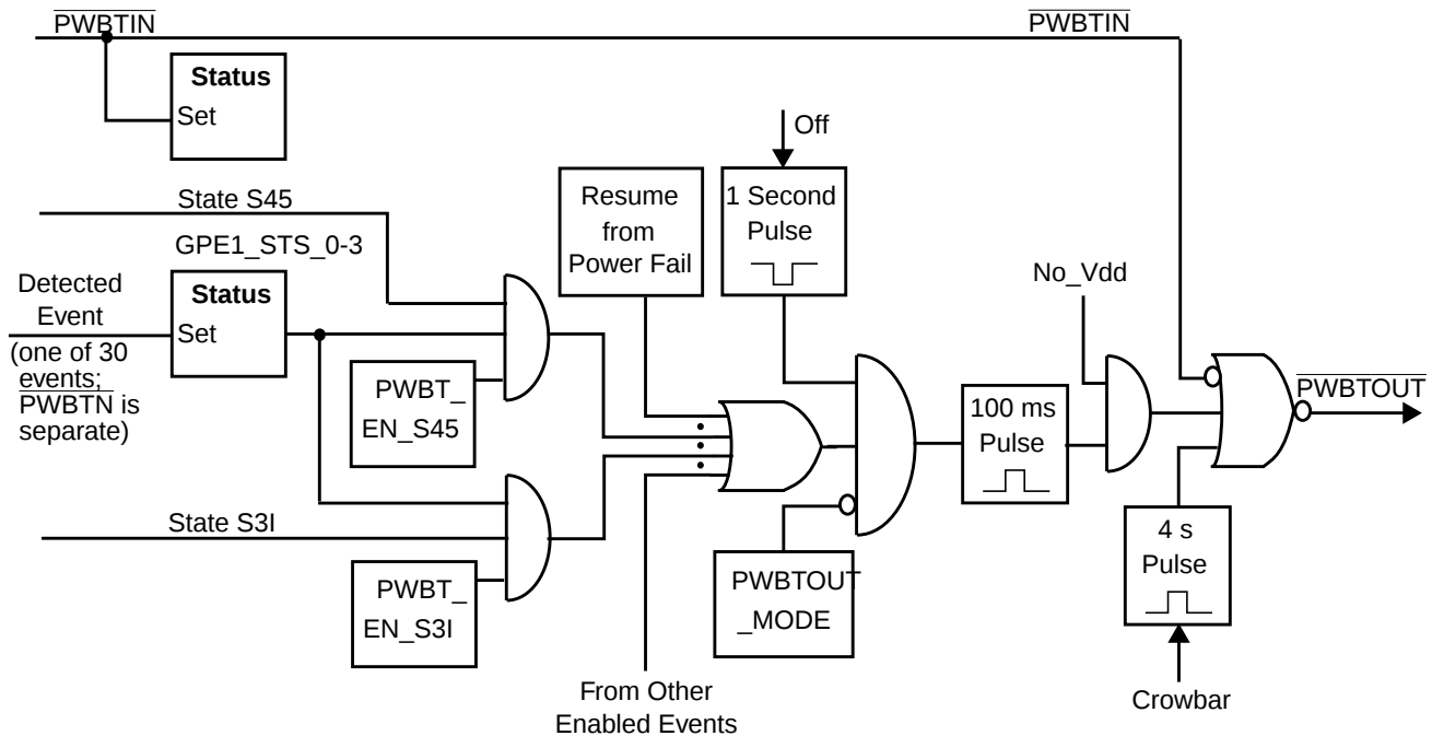
Figure 51. \overline{\text{PWBTOUT}} Control
