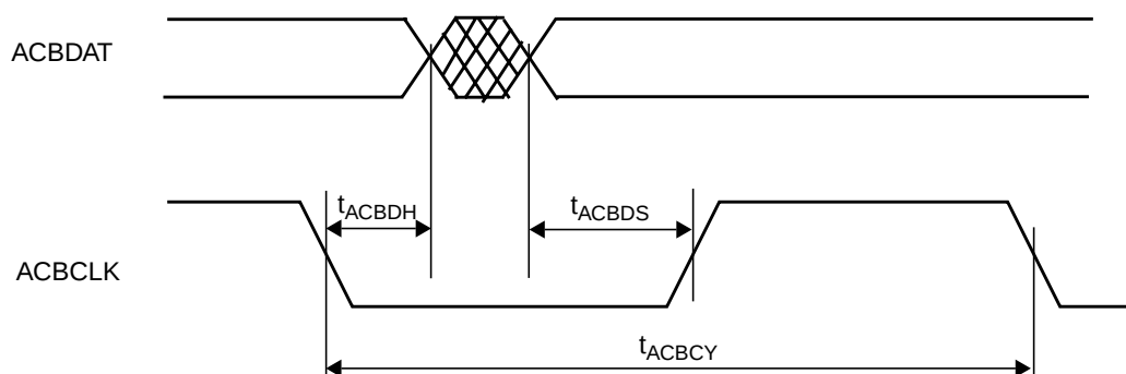
Figure 64. ACCESS.bus Data Bit Timing
