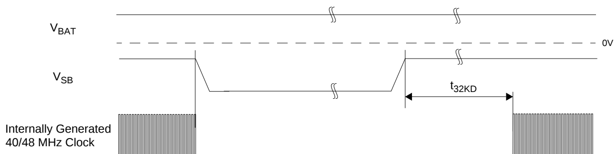
Figure 62. Internal Clock Waveforms
