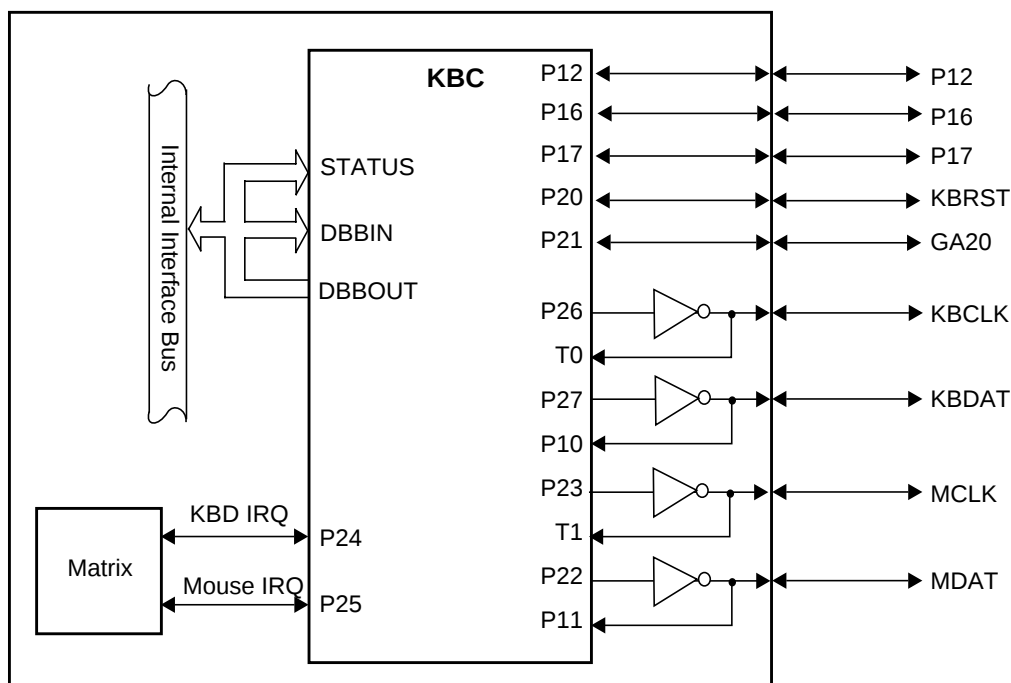
Figure 53. Keyboard and Mouse Interfaces
