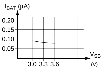
Figure 45. Typical Battery Current During Normal Operation Mode
