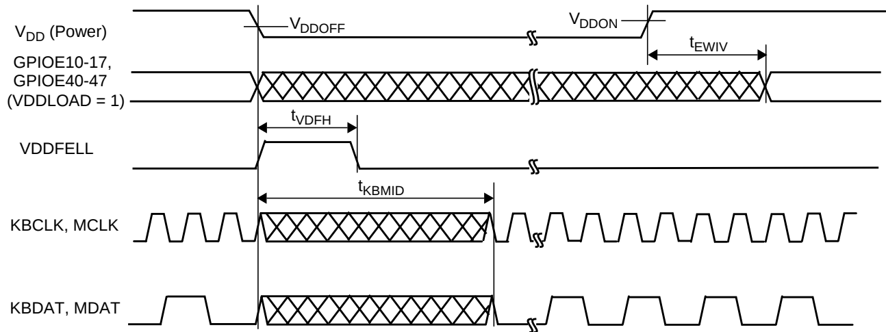
Figure 69. Wake-Up Inputs at V_{DD} Power Switching ( VDDFELL Enabled)
