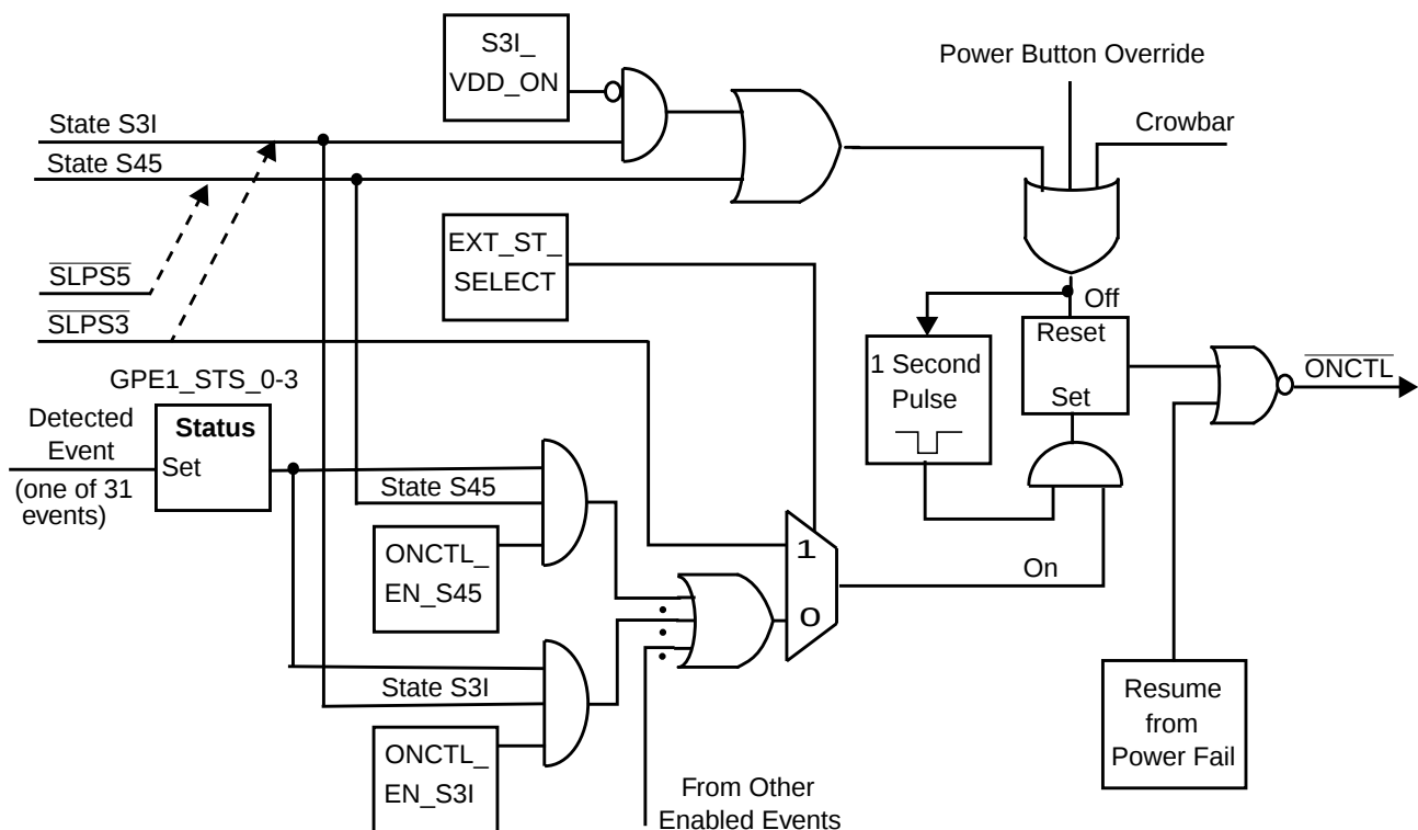
Figure 50. \overline{ONCTL} Control
