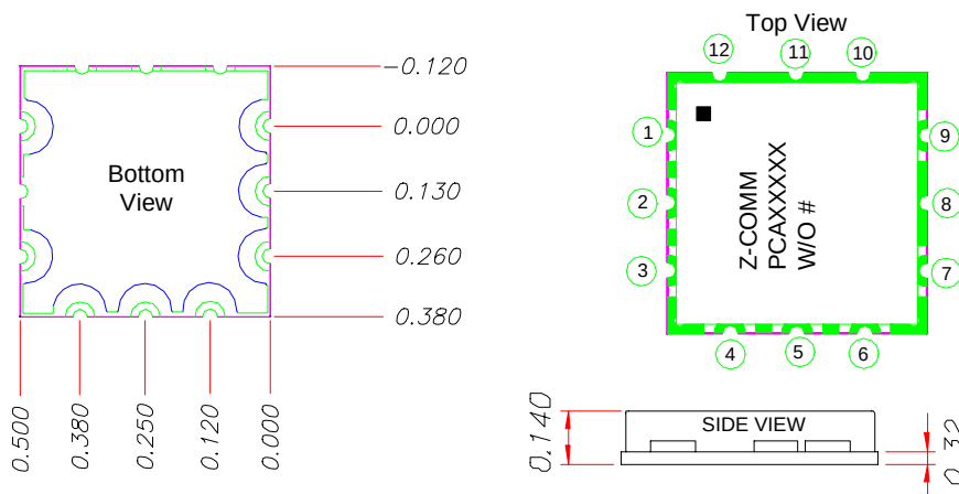
PHYSICAL DIMENSIONS
