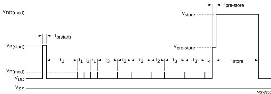
Fig.8 Supply voltage modulation for programming.
