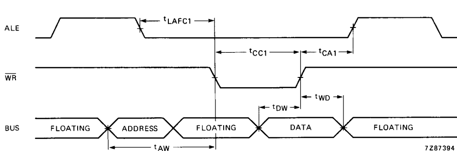
Fig.15 Write to external data memory.
