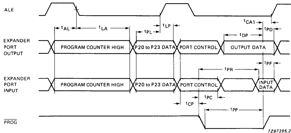
Fig.17 Port 2 timing
