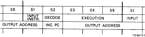
Fig. 11 Instruction cycle.
