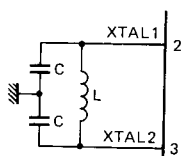
Fig. 7 LC oscillator mode
