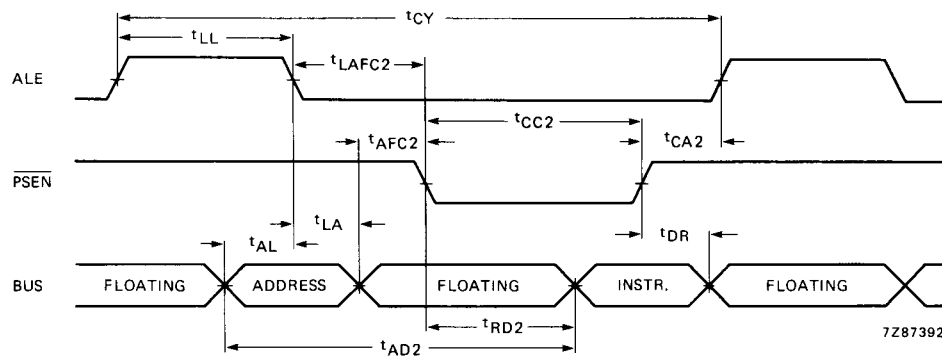
Fig.16 Instruction fetch from external program memory.
