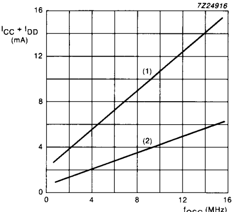
Fig.13 Typical values of maximum supply current ( I_{CC} + I_{DD} ) as a function of the oscillator frequency ( f_{OSC} ) at V_{CC}(\text{max.}) = 5.5\text{ V} ; T_{amb} = 0\text{ to }+70\text{ }^{\circ}\text{C}
