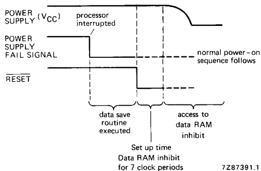
Fig. 9 Power-down sequence.
