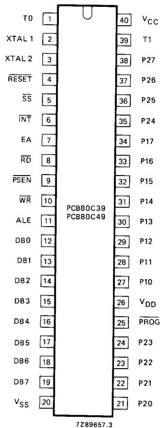
Fig. 2(a) Pinning diagram, DIL; for pin designation see next page.
