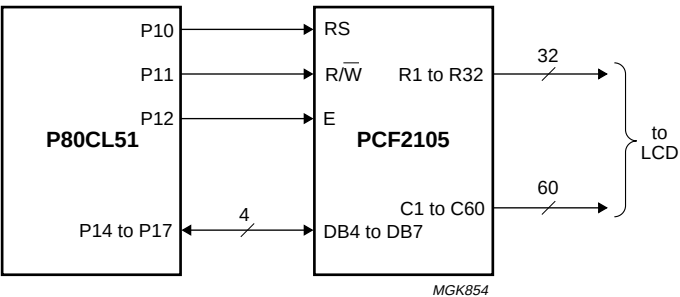
Fig.27 Direct connection to 8-bit microcontroller; 4-bit bus.
