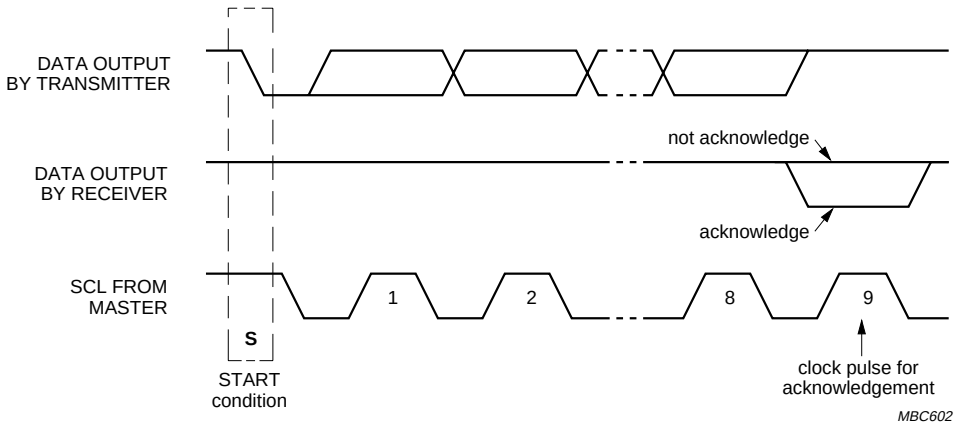
Fig.19 Acknowledgement on the I 2 C-bus.
