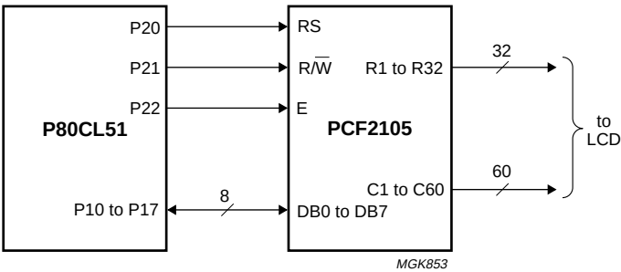
Fig.26 Direct connection to 8-bit microcontroller; 8-bit bus.
