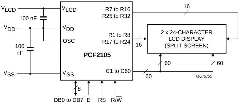
Fig.28 Typical application using parallel interface.
