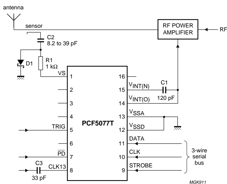
Fig.10 Application diagram for mobile stations.
