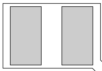
b. Outline of 1.2 mm 2 2 × 1 array giving 60% solder paste coverage.
