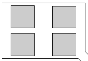
a. Outline of 0.4 mm 2 2 × 2 array giving 44% solder paste coverage.
