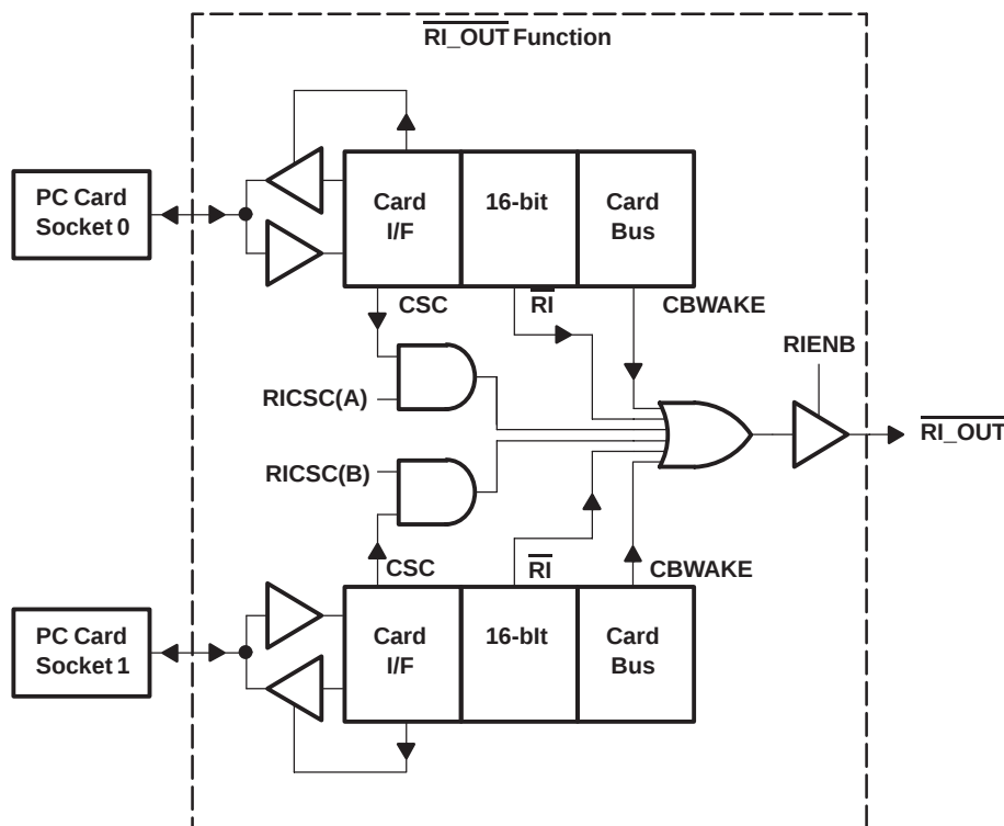
Figure 18. RI OUT Functional Illustration
