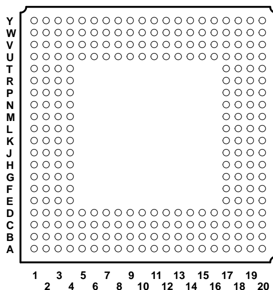
Figure 2-1. PCI1451 GFN Terminal Diagram
