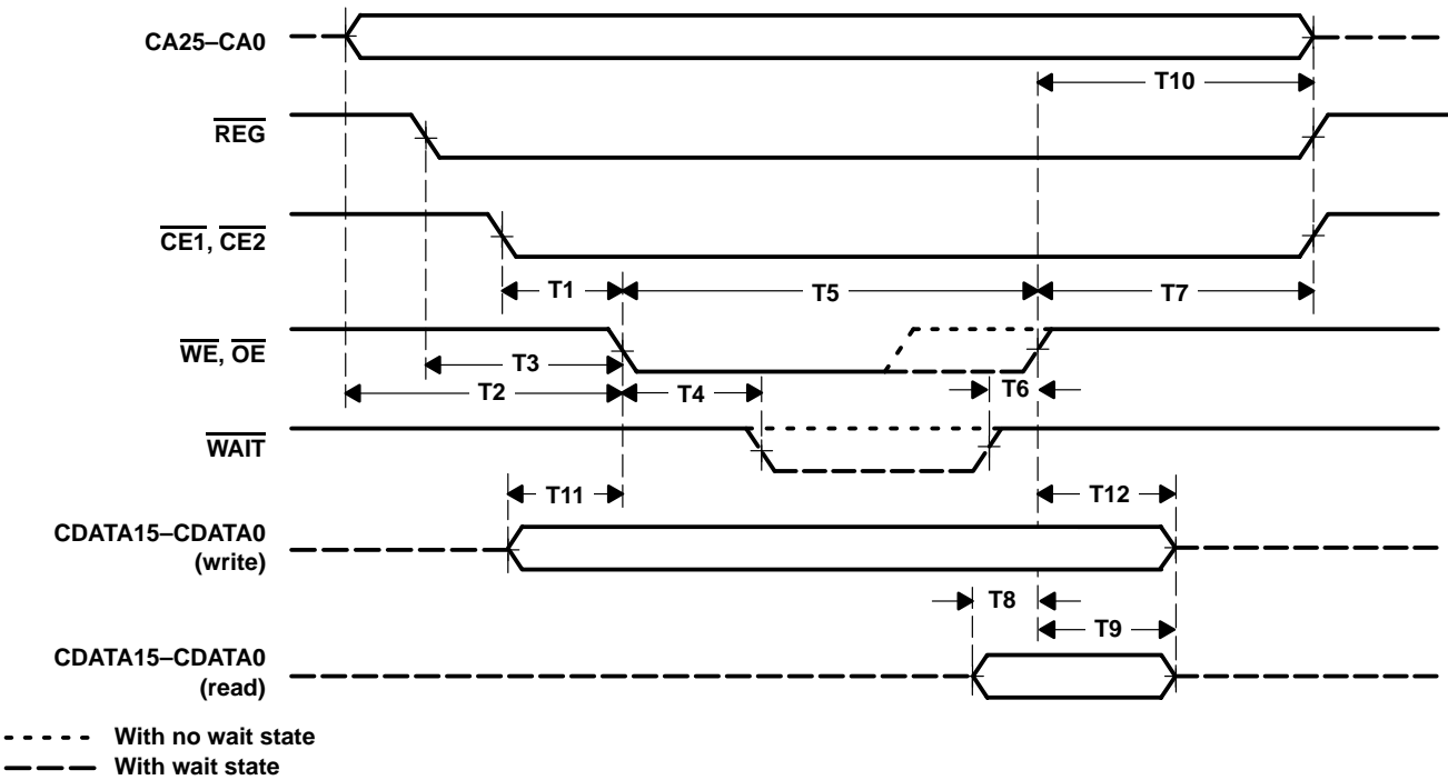
Figure 12–5. PC Card Memory Cycle
