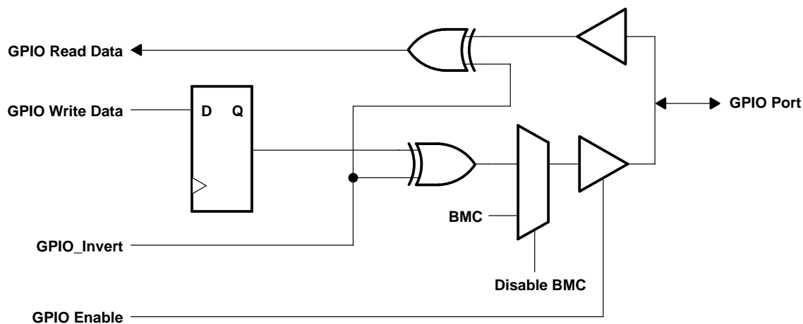
Figure 10–1. BMC/GPIO0
