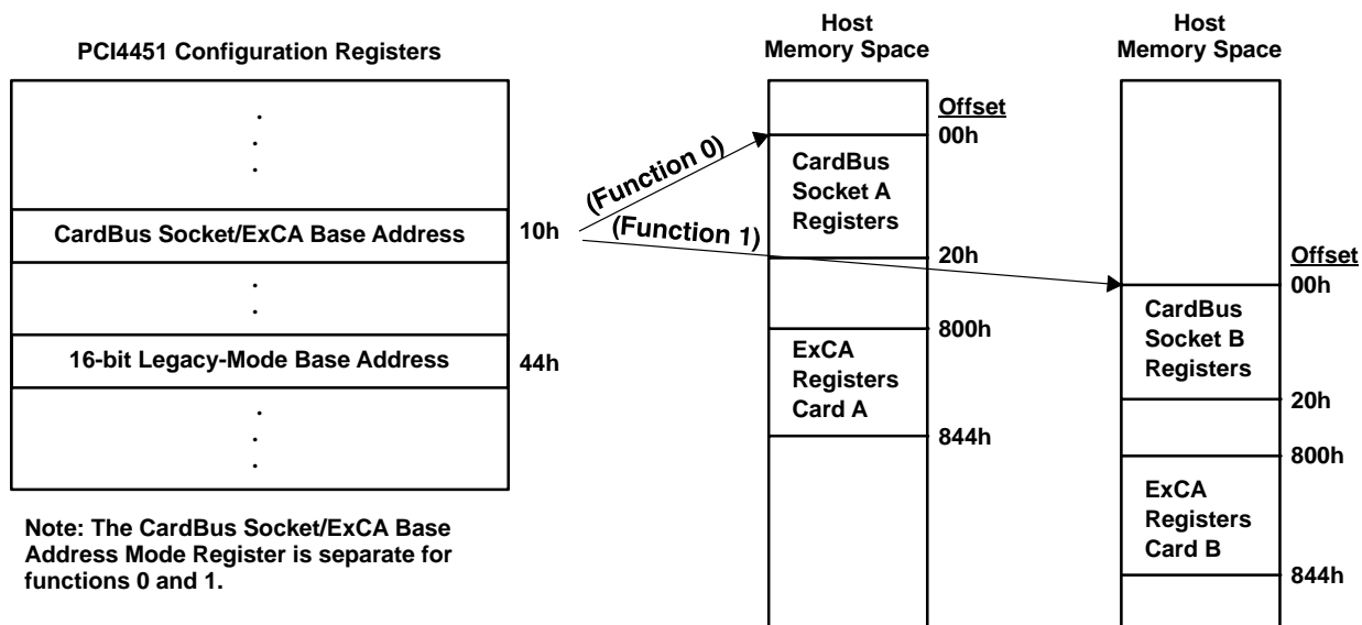
Figure 6–1. Accessing CardBus Socket Registers Through PCI Memory
