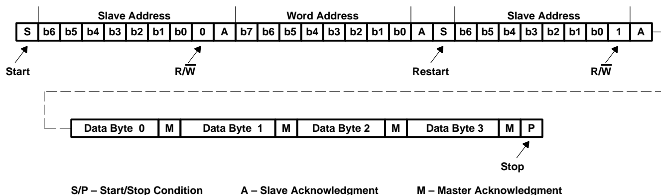
Figure 3-4. EEPROM Interface Subsystem Data Collection
