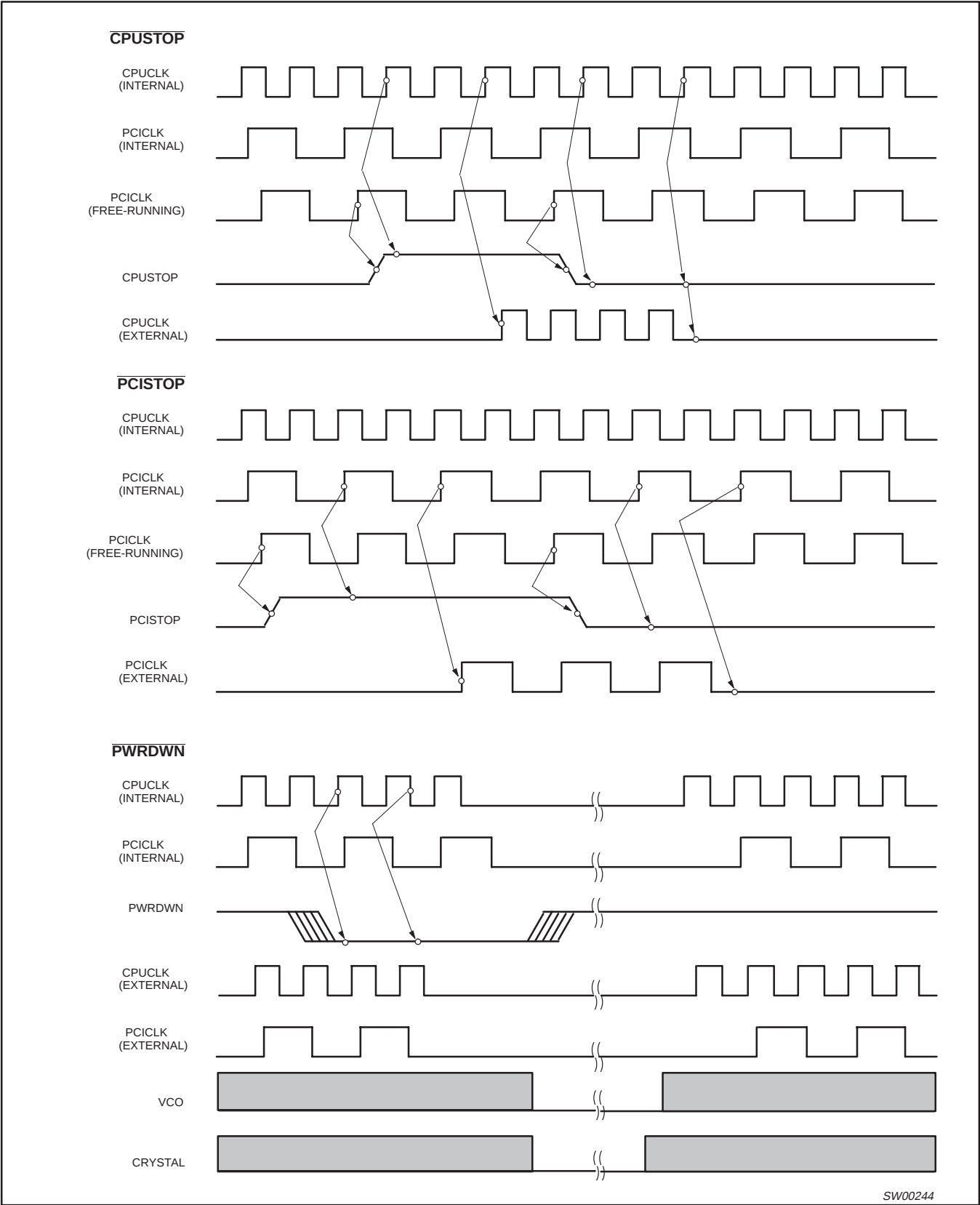
Figure 6. Power Management
