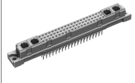
PCN11F-60S-2.54PFB-2 CL583-1187-7
