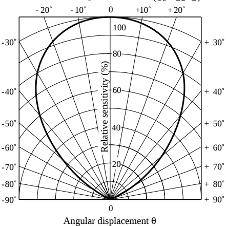
Fig. 8 Radiation Diagram (T a = 25°C)
