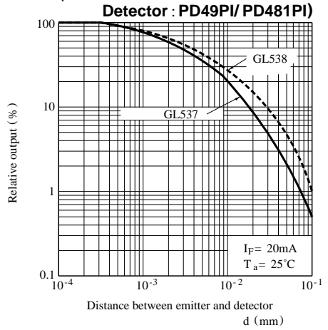
Fig. 8 Relative Output vs. Distance (Emitter:GL537/GL538)
