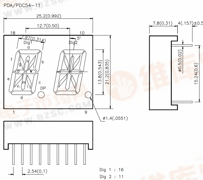
PDA54-11
