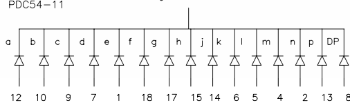
PDC54-11
