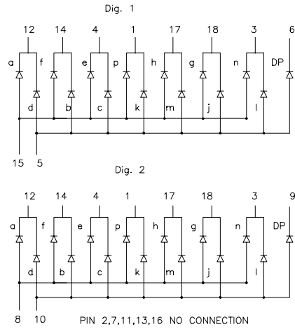
PDA54-12
