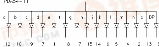
PDA54-11
