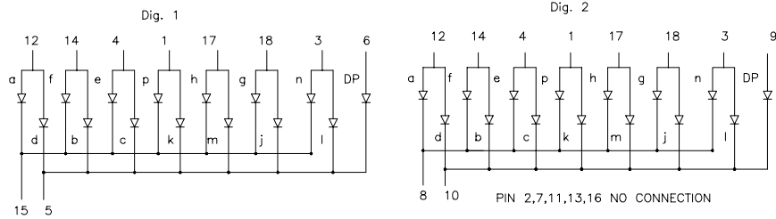
PDC54-12
