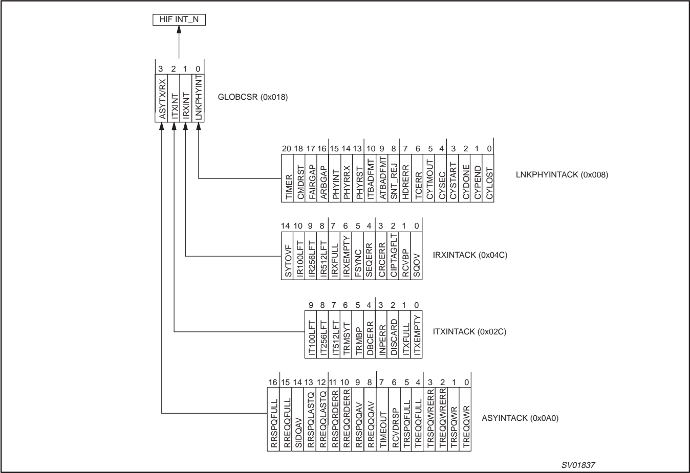
Figure 33. Interrupt Hierarchy
