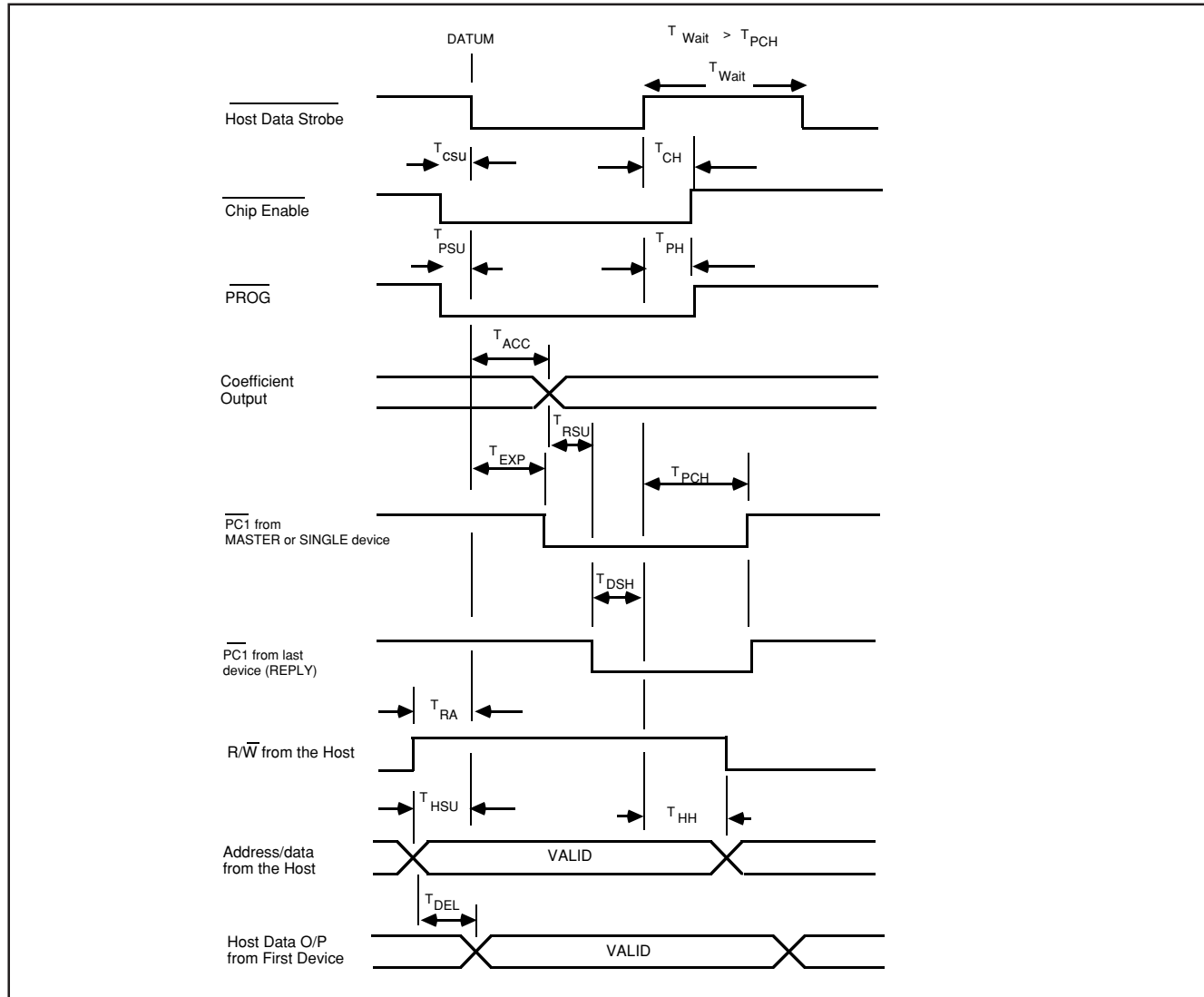
FIG. 8. Host Timing
