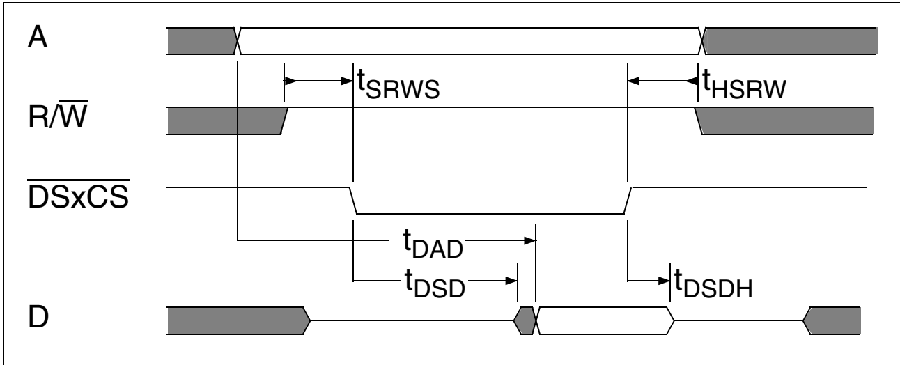
Figure 64 Read Cycle Motorola Mode
