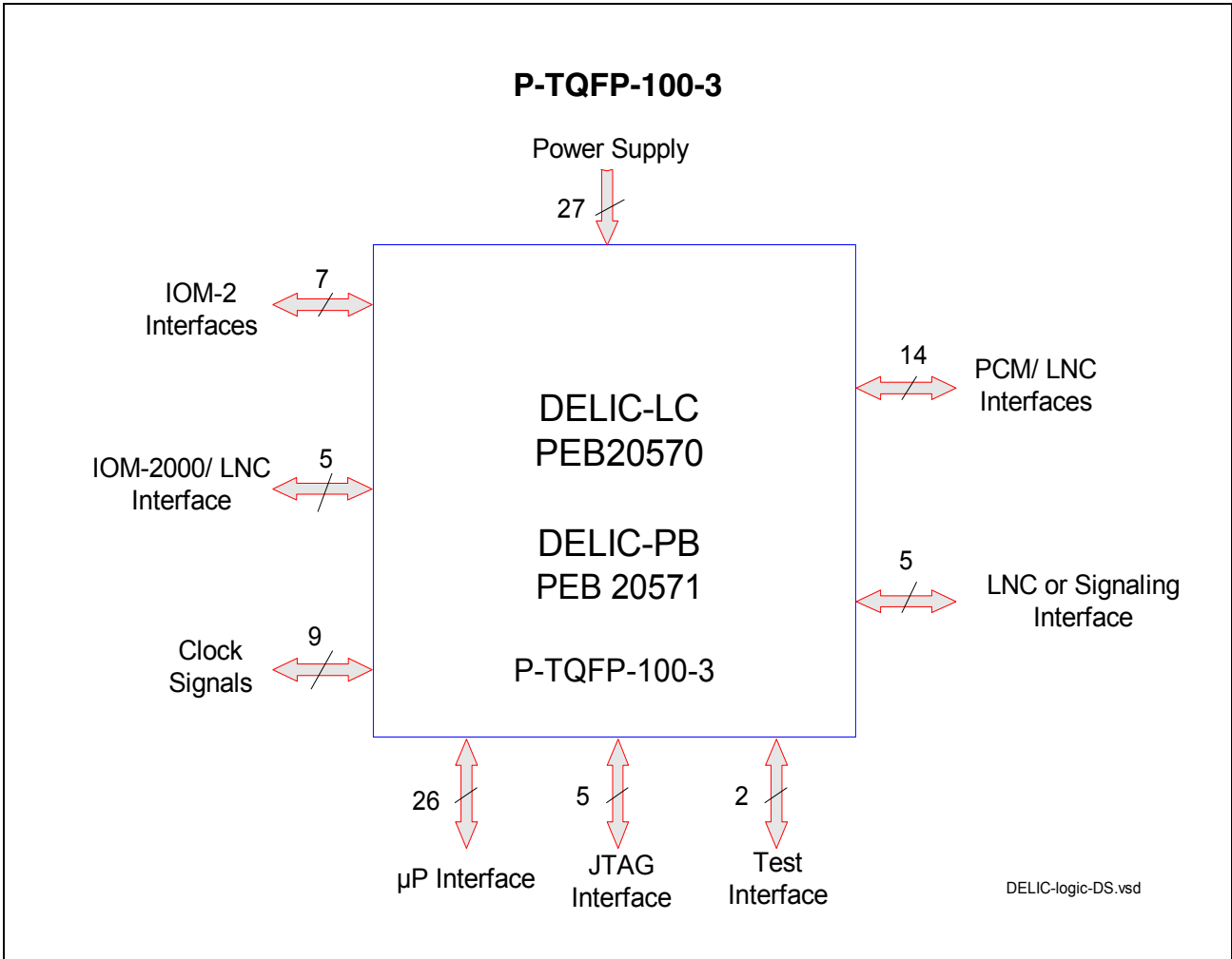
Figure 3 Logic Symbol
