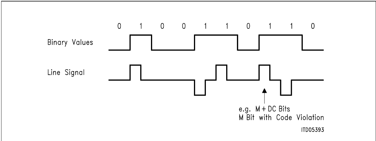
Figure 23 AMI Coding on the Up Interface
