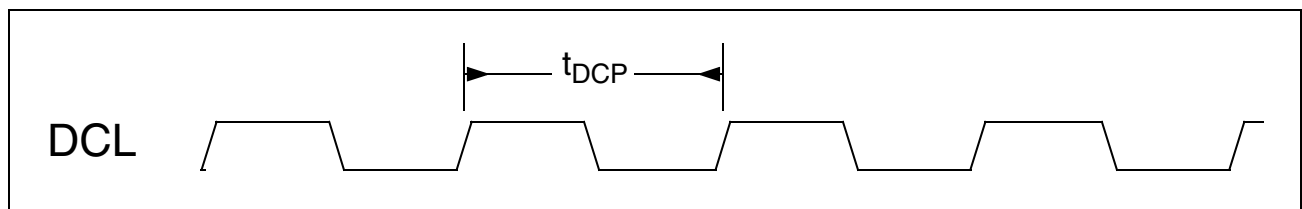
Figure 74 DCL Timing IOM-2
