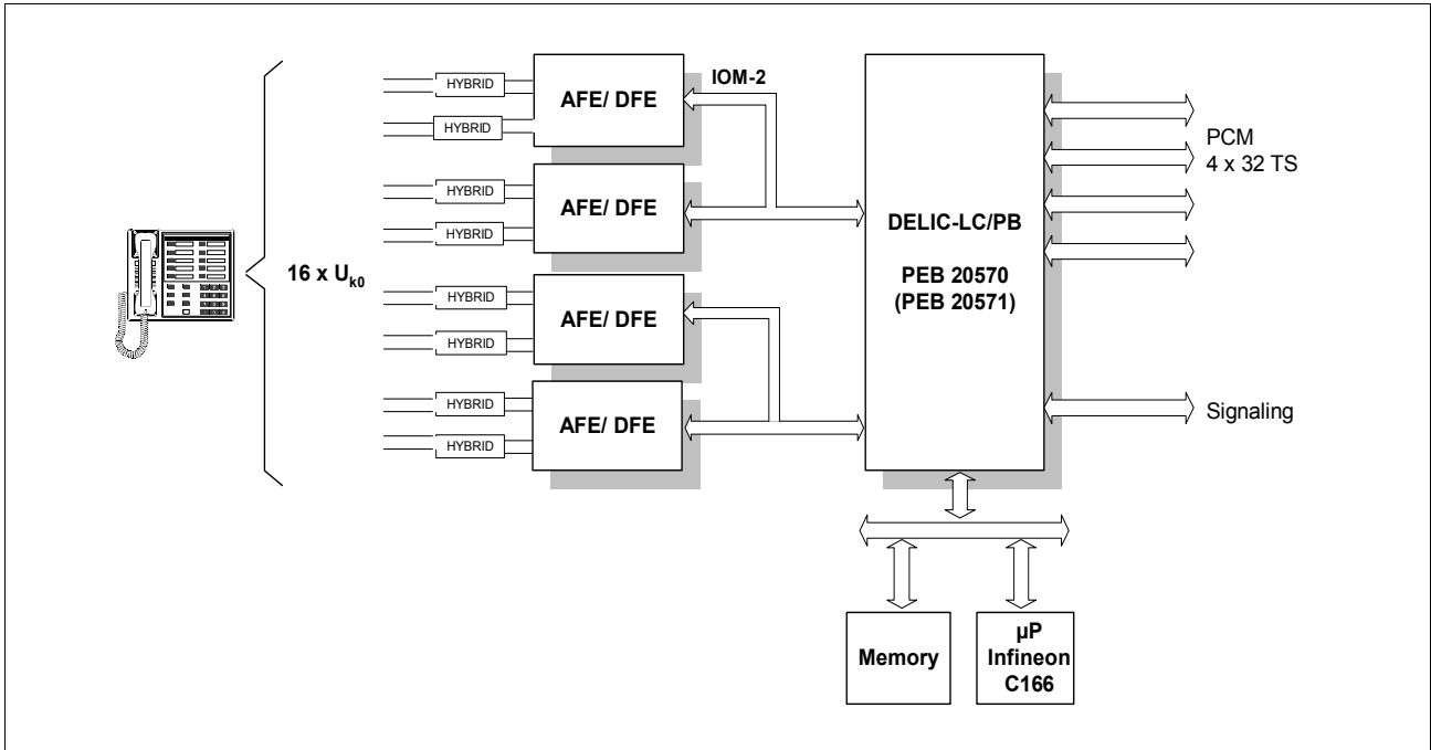
Figure 5 DELIC-LC/PB in Uko Line Card for 16 Subscribers
