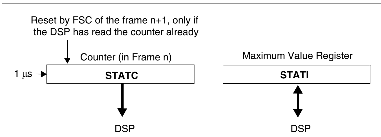
Figure 51 Statistics Registers
