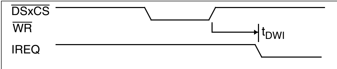
Figure 71 IREQ Deactivation Timing
