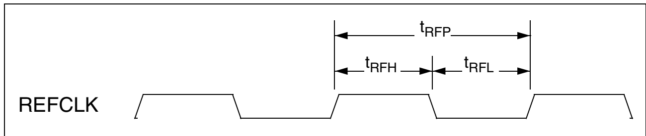
Figure 91 REFCLK Timing
