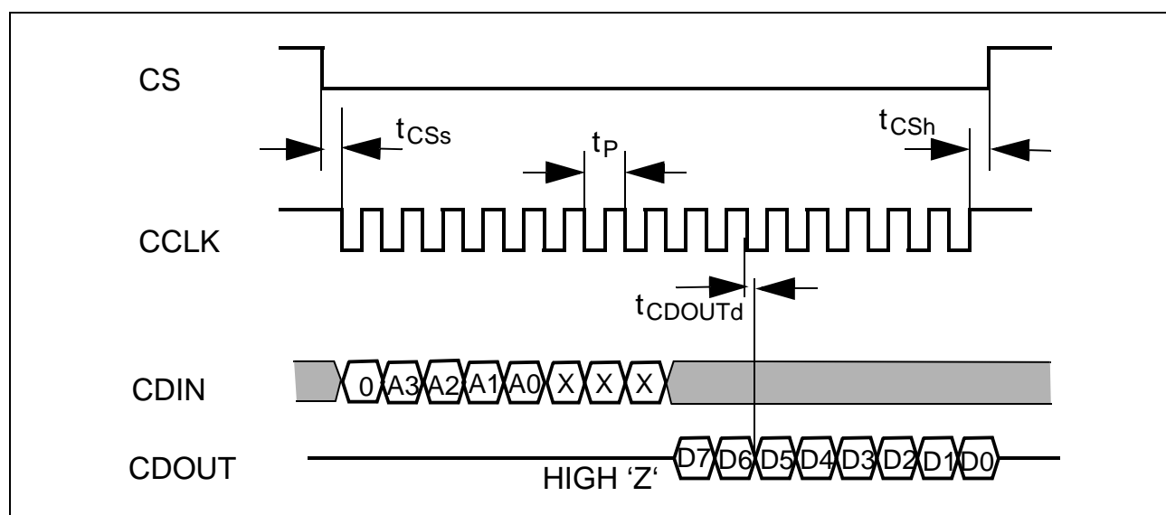
Figure 112 Serial μP Interface Mode Read
