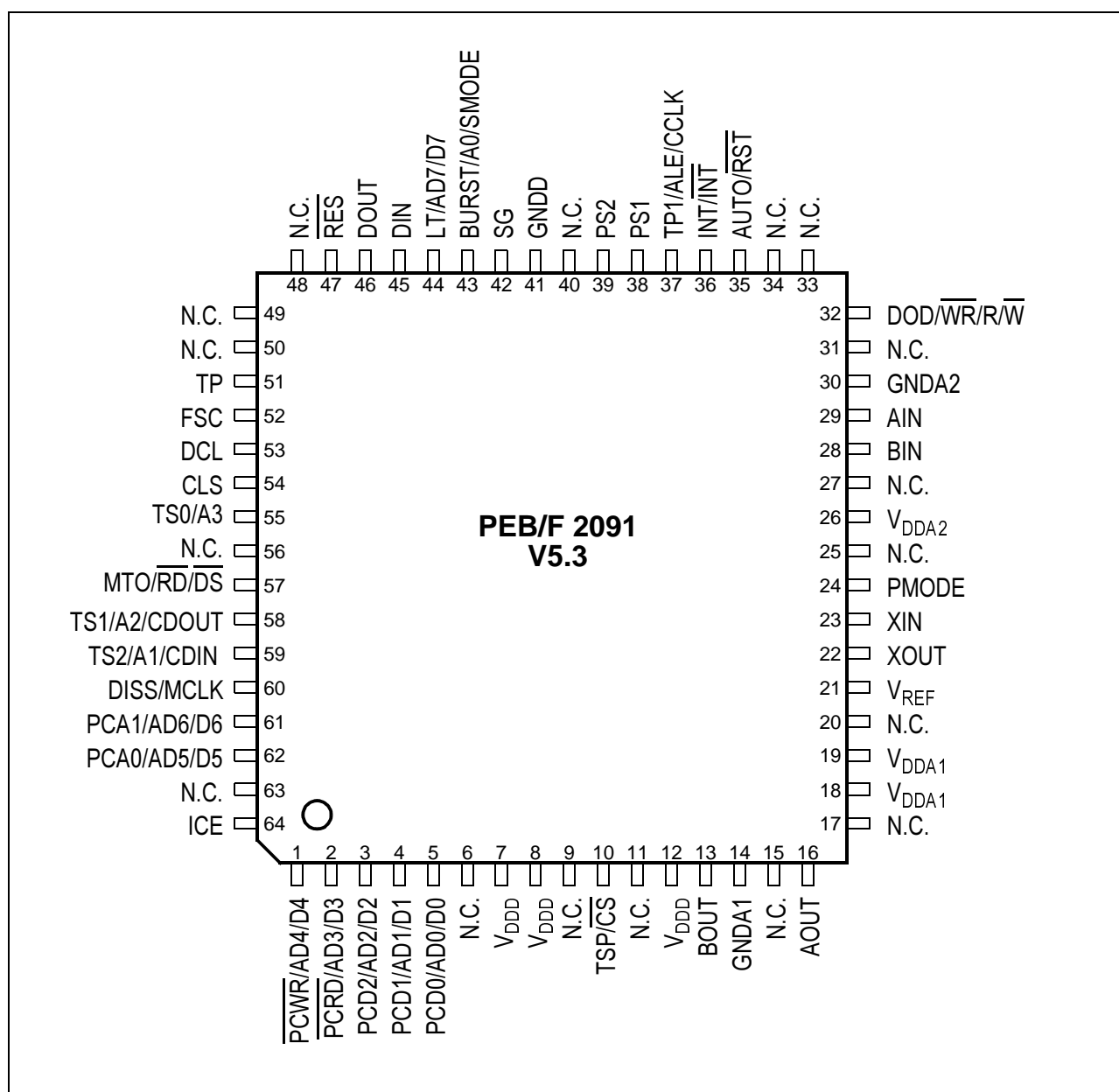
Figure 14 Pin Configuration for M-QFP-64 and T-QFP-64 Packages (top view)
