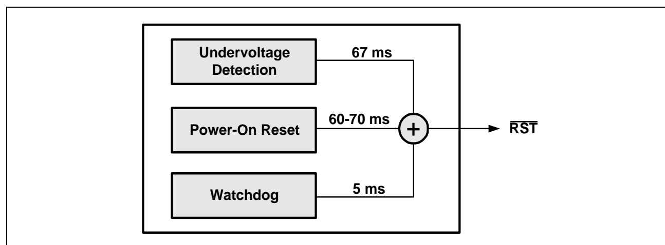
Figure 38 Reset Sources
