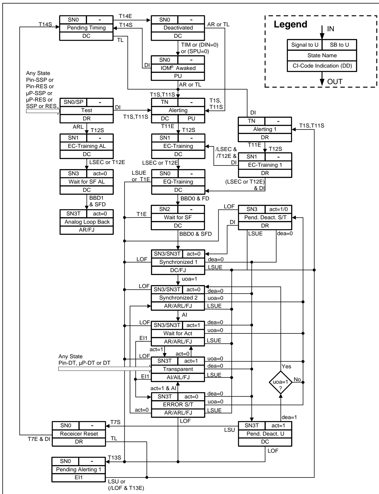
Figure 74 State Transition Diagram in NT-Auto Activation Mode
