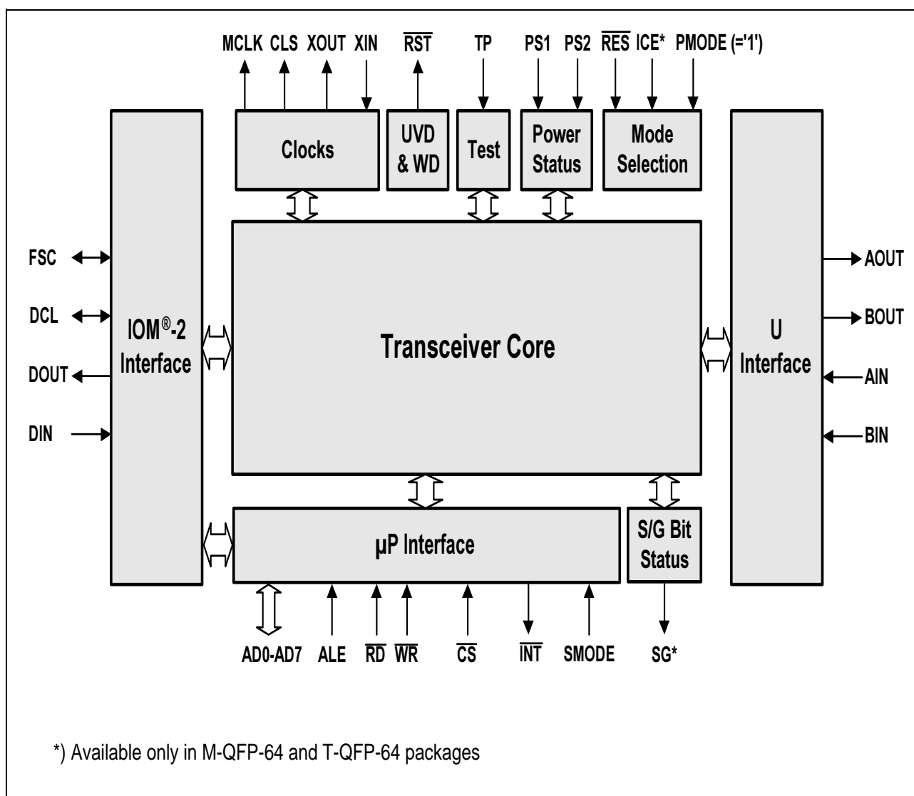
Figure 16 Device Architecture in µP Mode
