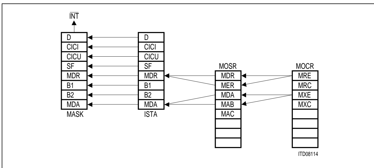
Figure 90 Interrupt Structure
