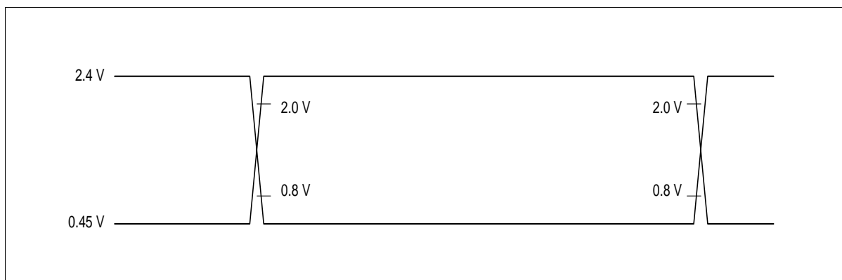
Figure 41 Input/Output Waveforms for AC-Tests
