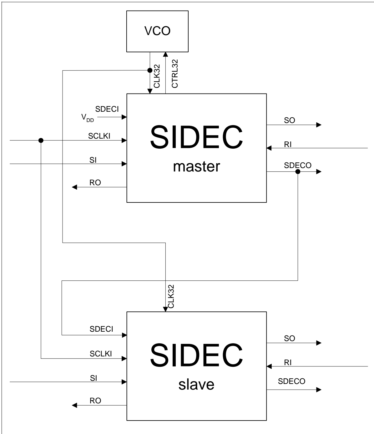
Figure 17 Multiple SIDECS
