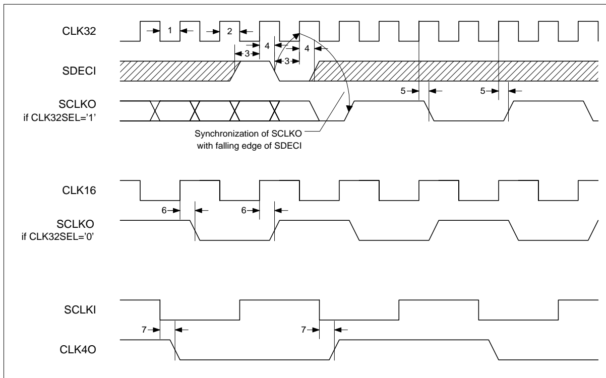
Figure 18 Clock Timing
