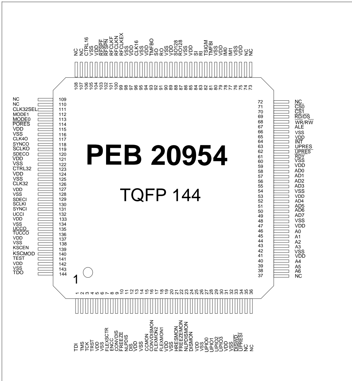
Figure 6 Pin Configuration
