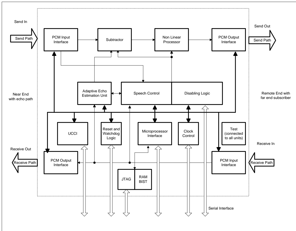
Figure 7 Block Diagram
