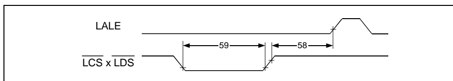
Figure 31 Read, Write, ALE Control Interval in Multiplexed Bus Mode
