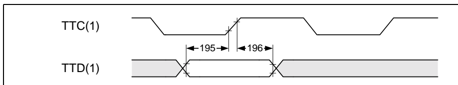
Figure 48 DS3 System Transmit Data Timing
