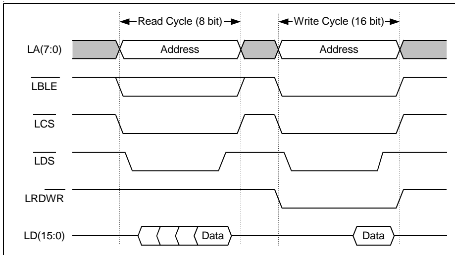
Figure 18 Motorola Bus Mode (Demultiplexed Bus Operation)
