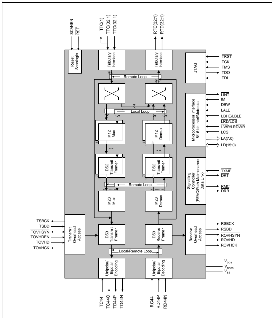
Figure 4 Block Diagram
