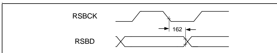
Figure 42 DS3 Receive Stuff Bit Timing
