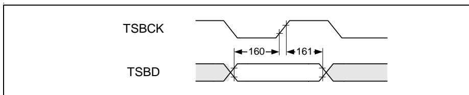
Figure 41 DS3 Transmit Stuff Bit Timing
