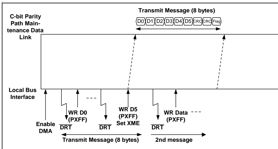
Figure 13 DMA supported Transmit Sequence
