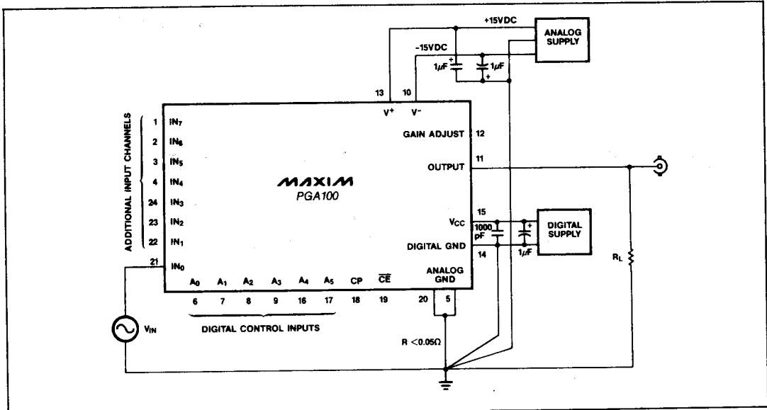
Figure 4. Basic Power Supply, Ground, and Signal Connections.
