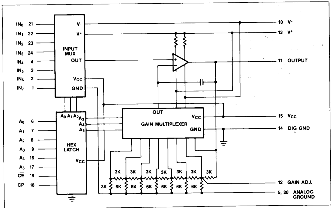
Figure 1. Equivalent Internal Schematic
