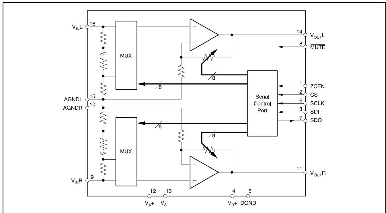
Figure 1. PGA2311 Block Diagram.
