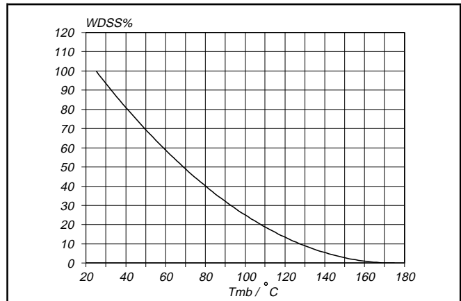
Fig.15. Normalised avalanche energy rating. W_{DSS}\% = f(T_{mb}) ; conditions: I_D = 40\text{ A}
