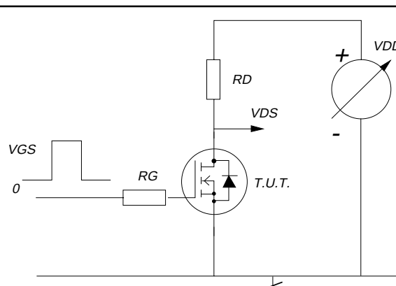
Fig.17. Switching test circuit.
