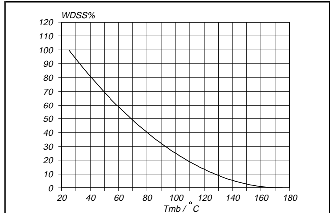
Fig.15. Normalised avalanche energy rating. W_{DSS}\% = f(T_{mb}) ; conditions: I_D = 75 A
