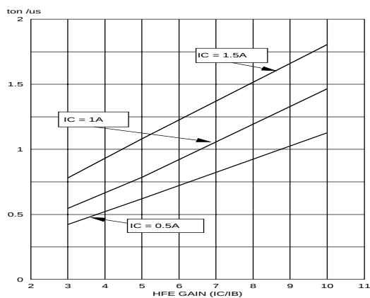
Fig.17. Resistive switching. t_{on} = f(h_{FE})
