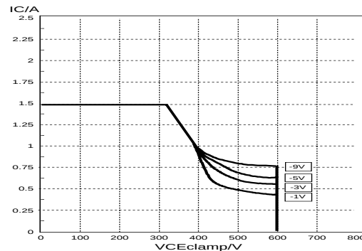
Fig.24. Reverse bias safe operating area T_j \leq T_{jmax} for -V_{BE} = 9V, 5V, 3V & 1V
