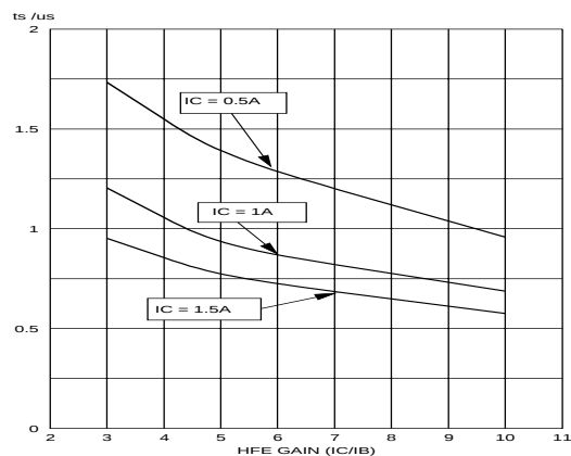
Fig.19. Resistive switching. t_s = f(h_{FE})
