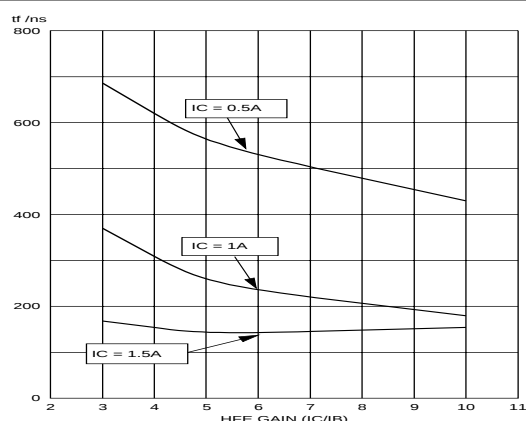
Fig.21. Resistive switching. t_f = f(h_{FE})
