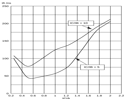
Fig.12. Inductive switching. t_{ft} = f(I_C)
