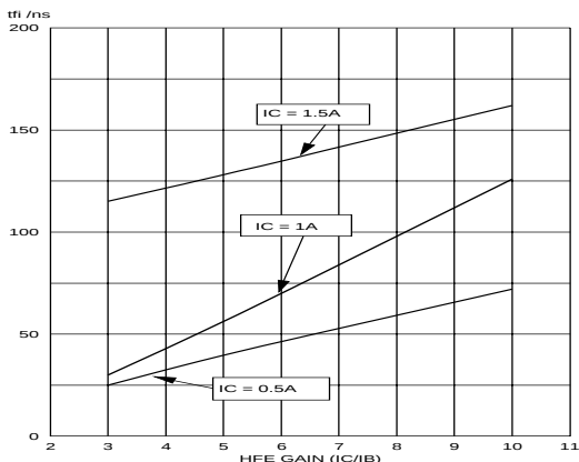
Fig.11. Inductive switching. t_{ft} = f(h_{FE})
