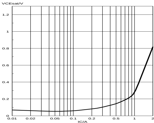
Fig.7. Collector-Emitter saturation voltage. Solid Lines = typ values, I_C/I_B = 3
