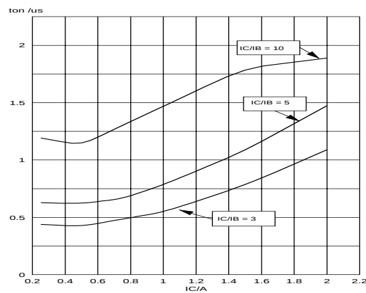
Fig.18. Resistive switching. t_{on} = f(I_C)
