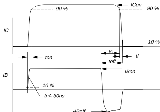
Fig.12. Switching times waveforms with resistive load.
