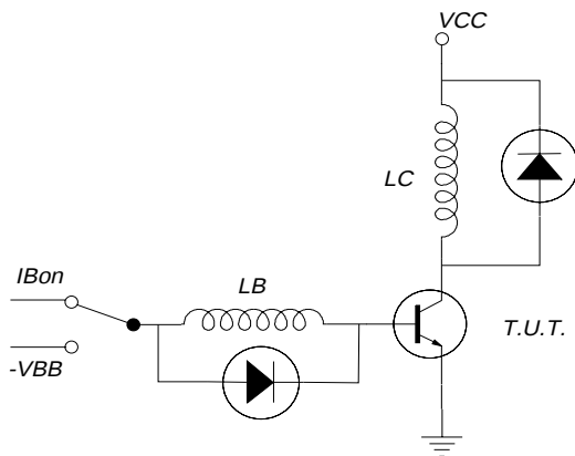
Fig.9. Test circuit inductive load. V_{CC} = 300 V; -V_{BE} = 5 V, L_C = 200 \mu H; L_B = 1 \mu H
