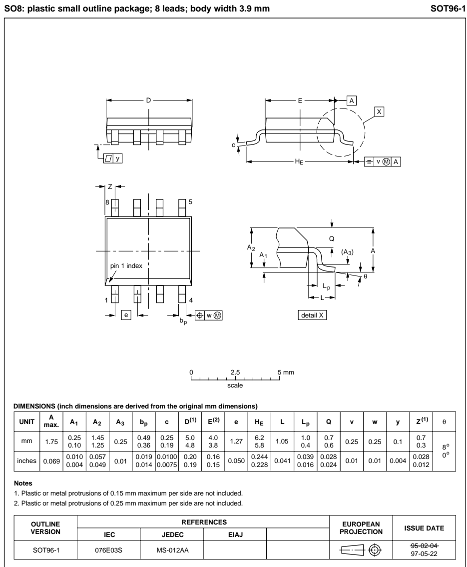
Fig. 15. SOT96 surface mounting package.
