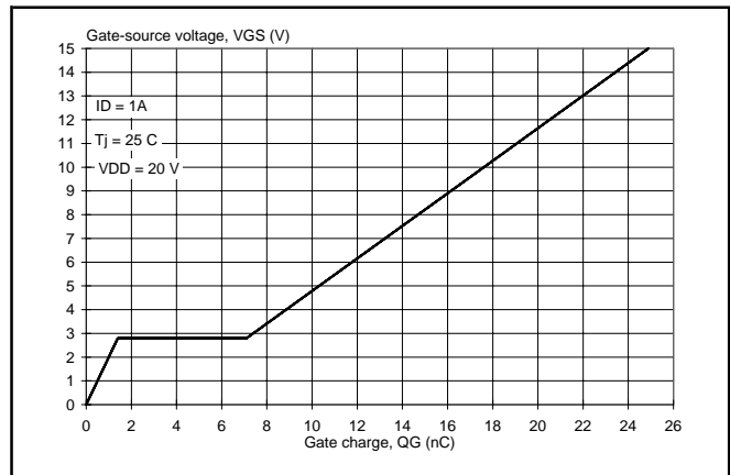
Fig.21. Typical turn-on gate-charge characteristics (isolation FET); V_{GS} = f(Q_G)
