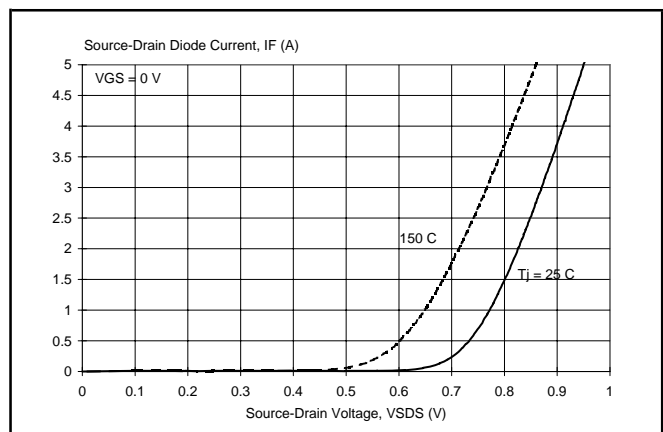
Fig.22. Typical reverse diode current (spindle FET) I_F = f(V_{SDS}); conditions: V_{GS} = 0\text{ V}; parameter T_j
