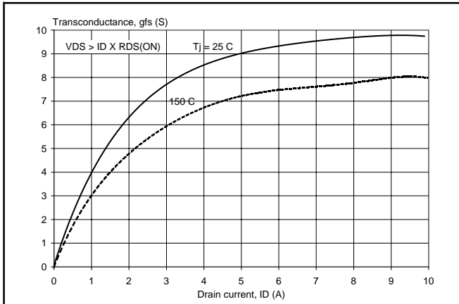
Fig.17. Typical transconductance (isolation FET) T_j = 25\text{ }^\circ\text{C}; g_{fs} = f(I_D)
