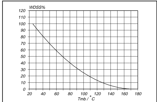
Fig.15. Normalised avalanche energy rating. W_{DSS}\% = f(T_{mb}) ; conditions: I_D = 32 A
