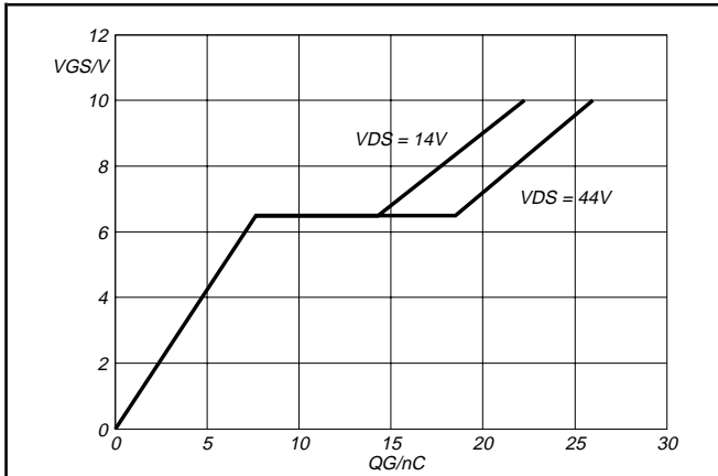
Fig.13. Typical turn-on gate-charge characteristics. V_{GS} = f(Q_G) ; conditions: I_D = 30 A; parameter V_{DS}
