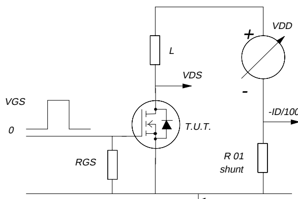
Fig.18. Unclamped inductive test circuit.
