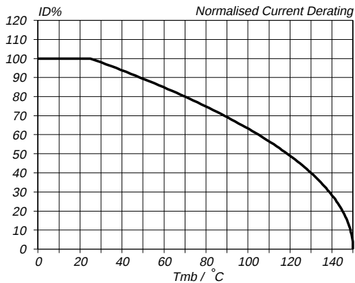
Fig.2. Normalised continuous drain current. ID\% = 100 \cdot I_D / I_{D 25\text{ }^\circ\text{C}} = f(T_{sp}) ; conditions: V_{GS} \geq 10\text{ V}
