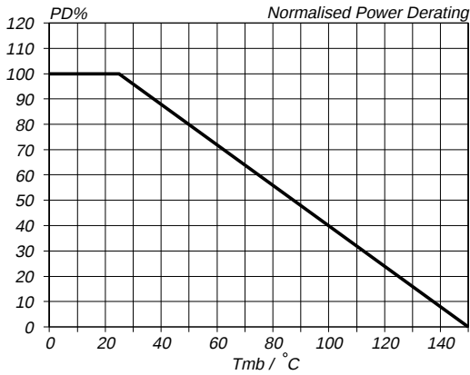
Fig.1. Normalised power dissipation. PD\% = 100 \cdot P_D / P_{D 25\text{ }^\circ\text{C}} = f(T_{sp})
