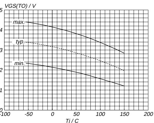
Fig.10. Gate threshold voltage. V_{GS(T0)} = f(T_j) ; conditions: I_D = 1 mA; V_{DS} = V_{GS}
