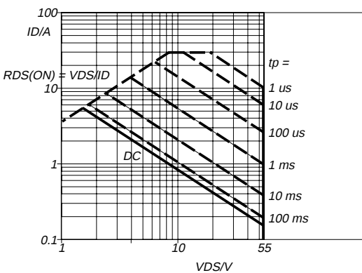
Fig.3. Safe operating area. T_{sp} = 25\text{ }^\circ\text{C} I_D \text{ \& } I_{DM} = f(V_{DS}) ; I_{DM} single pulse; parameter t_p
