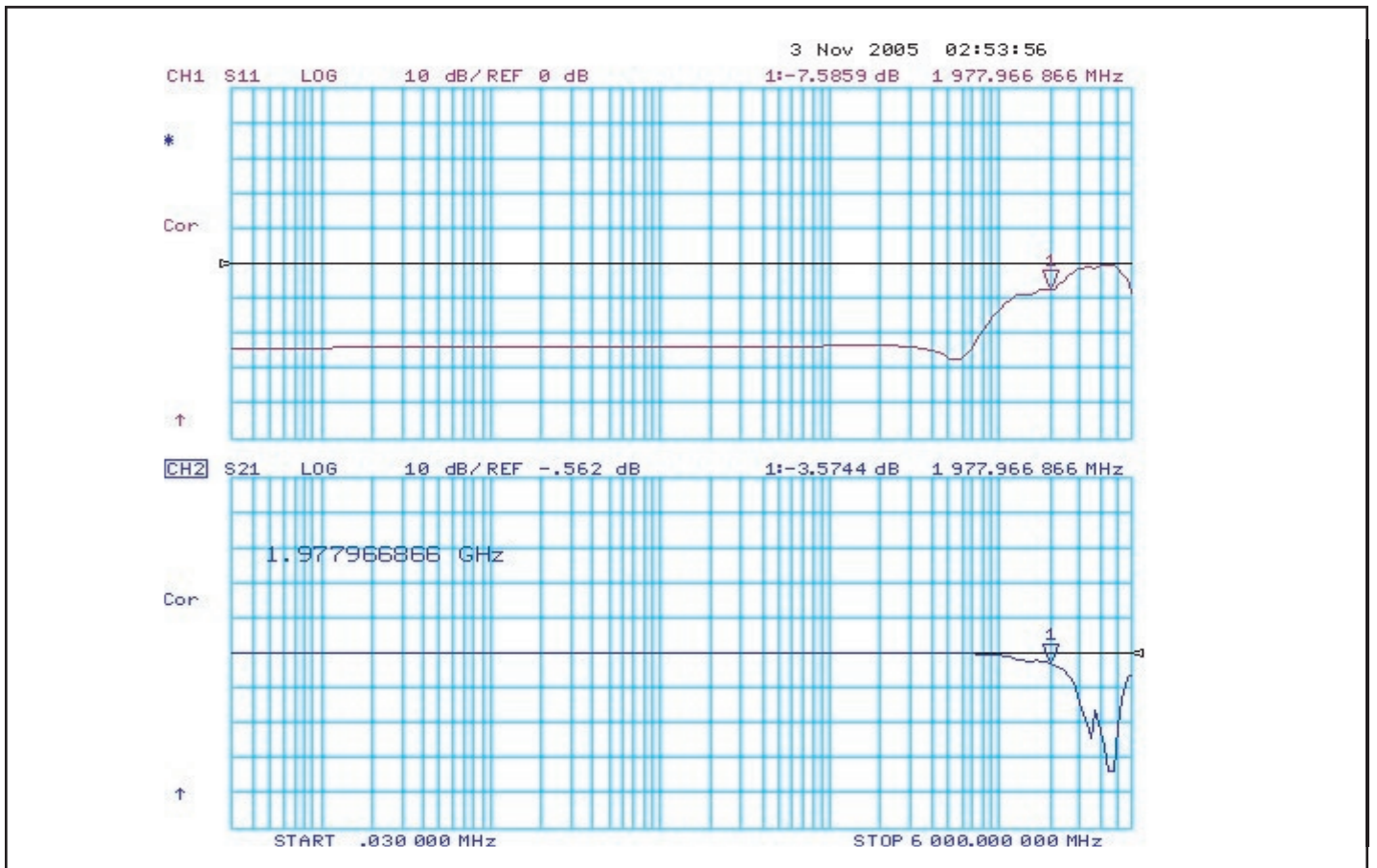
Fig 8. Return and Insertion Loss Log Diagram from 30kHz to 6.0GHz using Matching Cables, Vcc=1.8V, 25C
