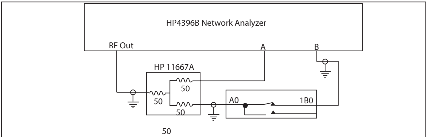
Fig 3. Bandwidth Setup
