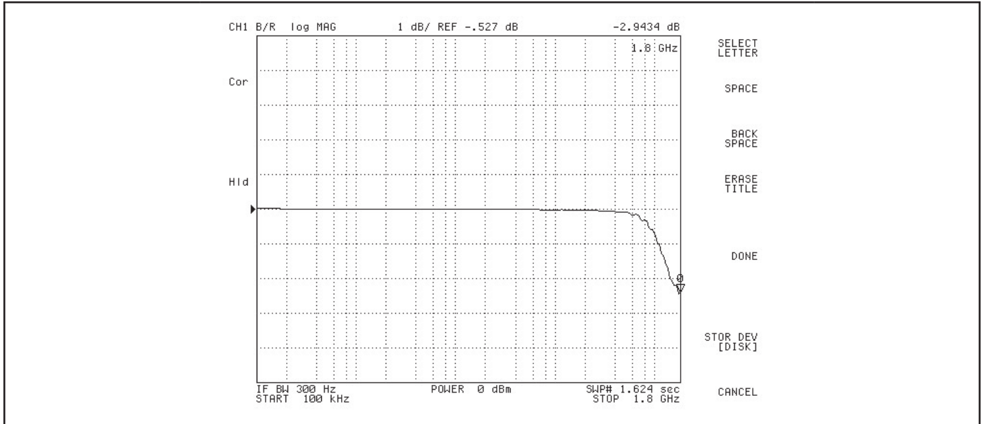
Fig 7. -3 dB Bandwidth, Vcc=1.8V, 25°C
