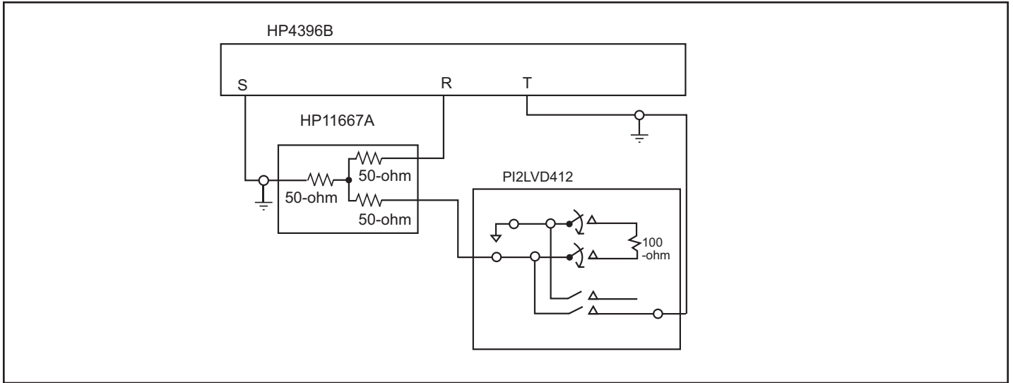
Fig 2. Off-isolation setup
