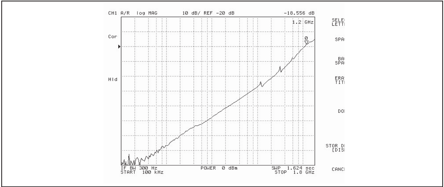
Fig 5. Crosstalk, V_{CC} = 1.8V , 25^{\circ}C
