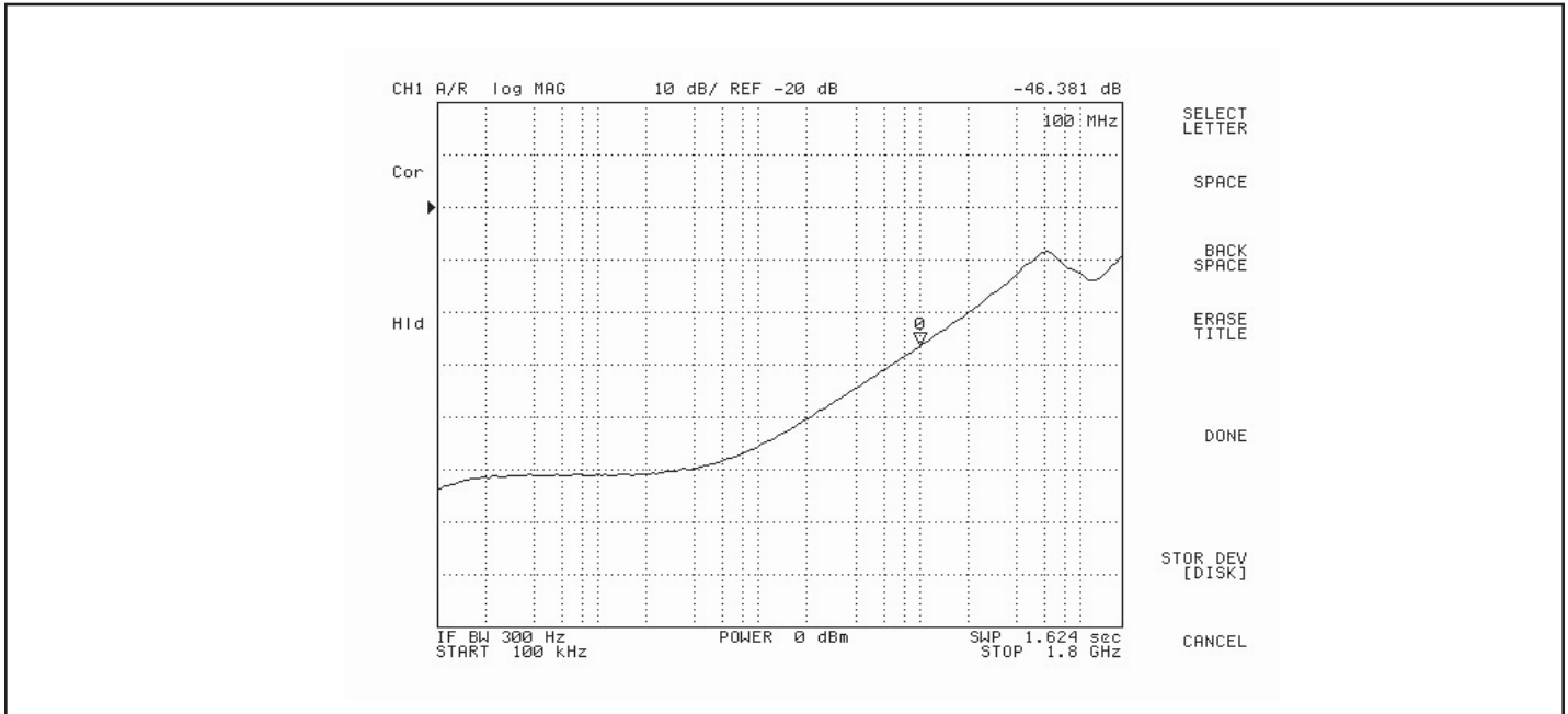
Fig 6. Off Isolation, V_{CC} = 1.8V , 25^{\circ}C
