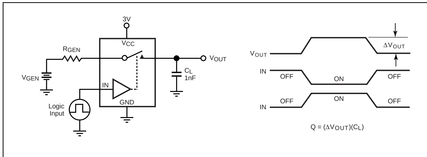
Figure 3. Charge Injection
