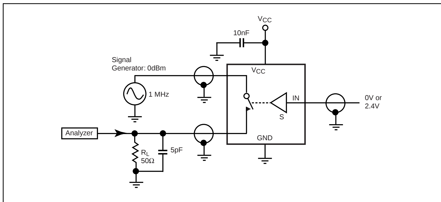
Figure 4. Off Isolation
