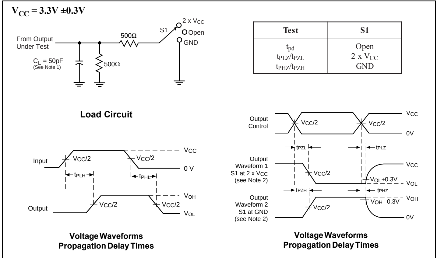
Figure 2. Test Circuit and Voltage Waveforms for V_{CC} = 3.3V
