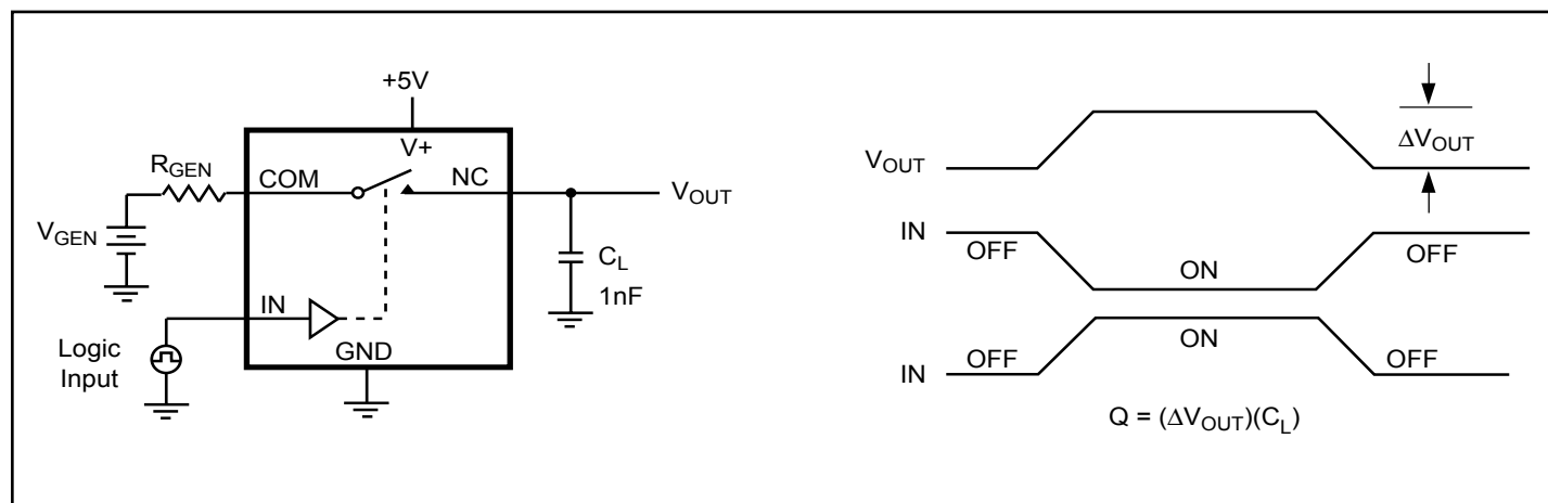
Figure 2. Charge Injection
