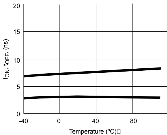
Switching Times vs. Temperature
