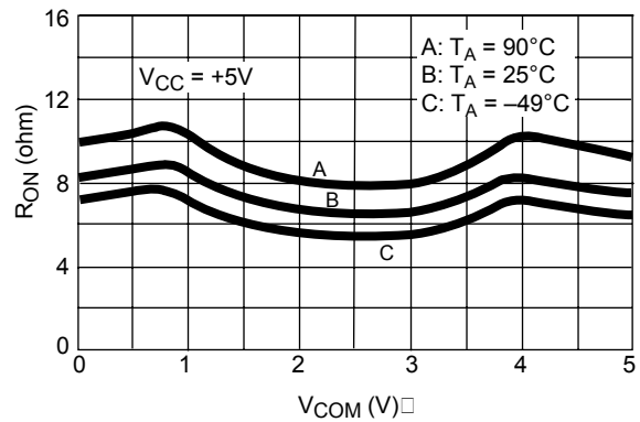
R_{ON} vs. V_{COM} and Temperature
