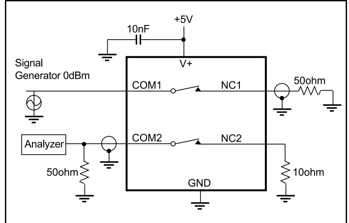
Figure 4. Crosstalk (124 only)
