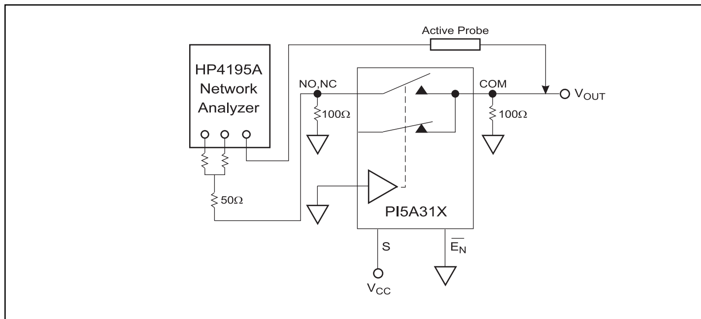
Figure 3. Bandwidth
