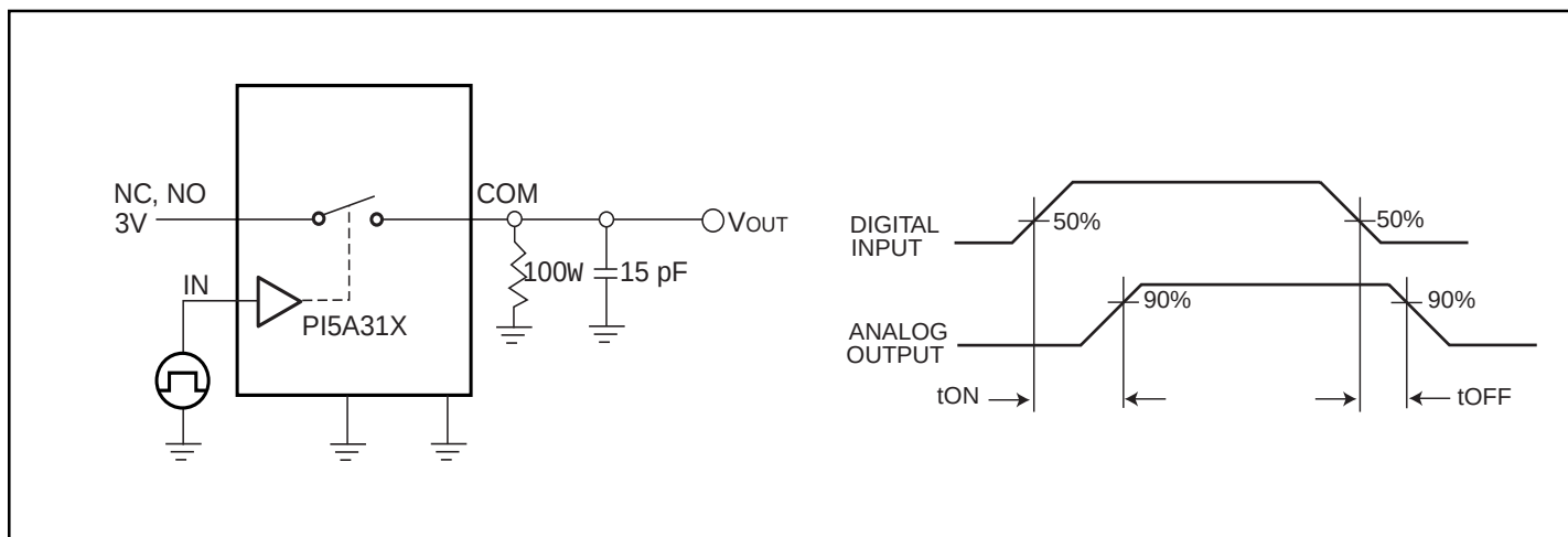
Figure 1. Switching Time
