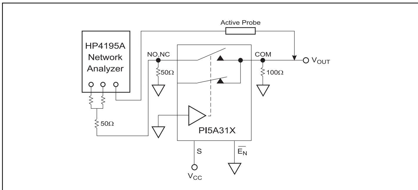
Figure 2. Off Isolation
