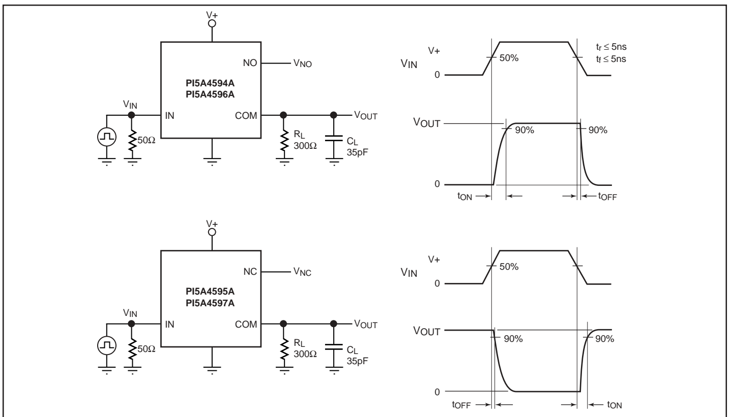
Figure 3. Switching Times
