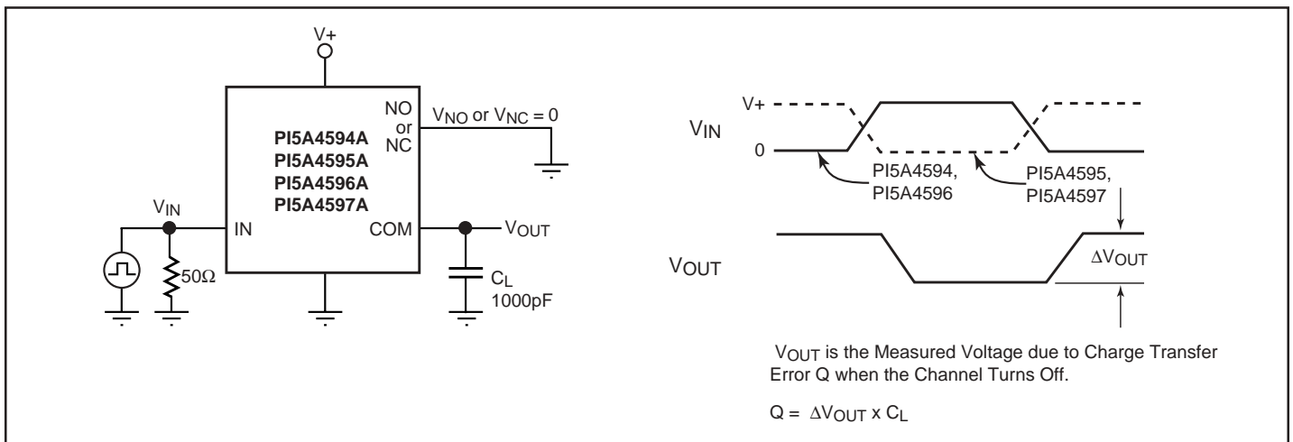
Figure 2. Charge Injection
