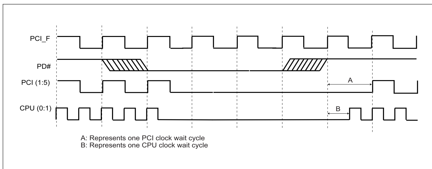
Figure 1. PD# Timing Diagram
