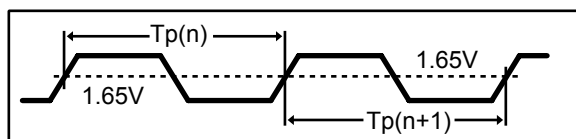
Figure 4. Cycle jitter
