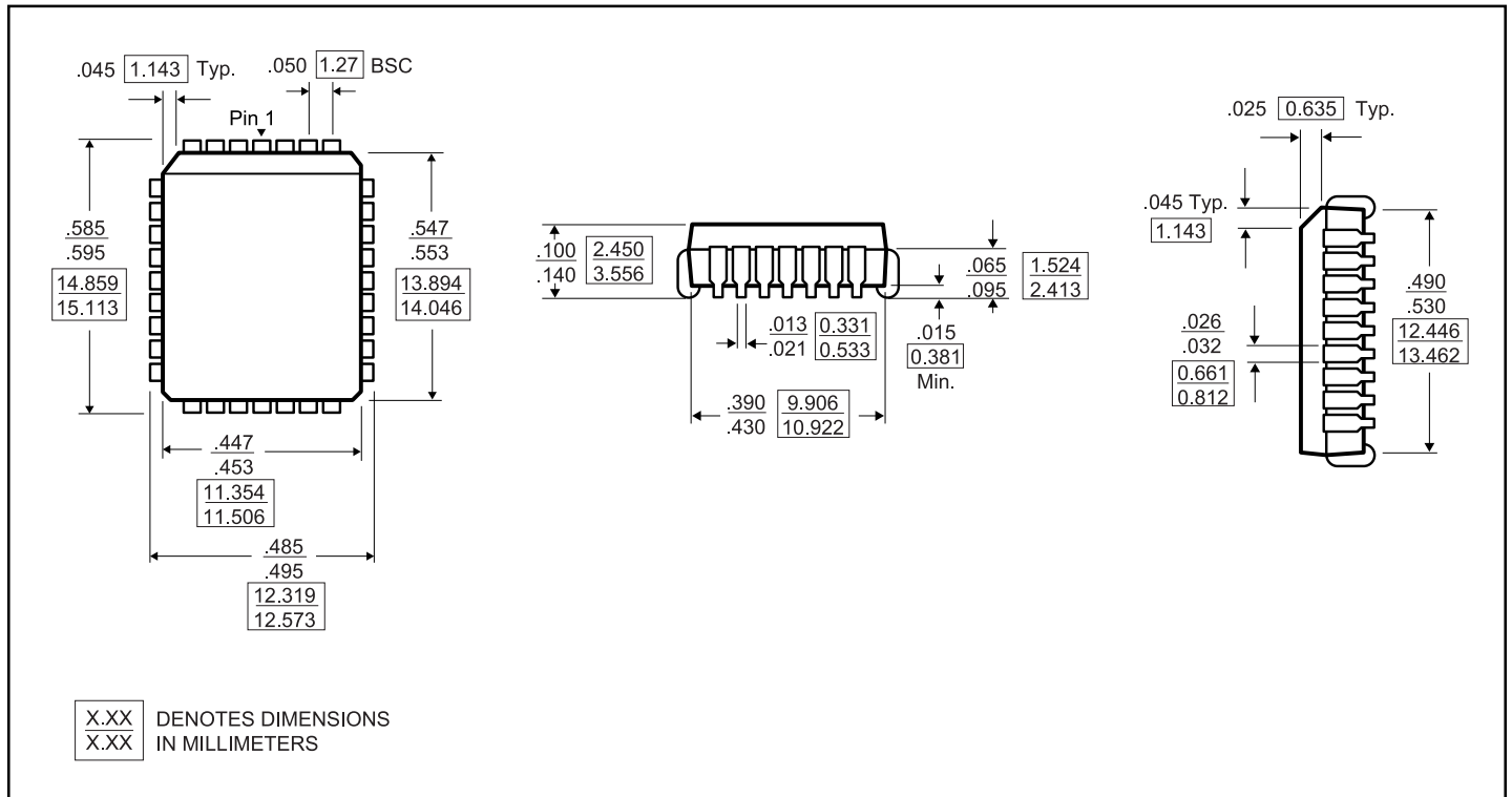
Package Diagram - 32-Pin PLCC (J)
