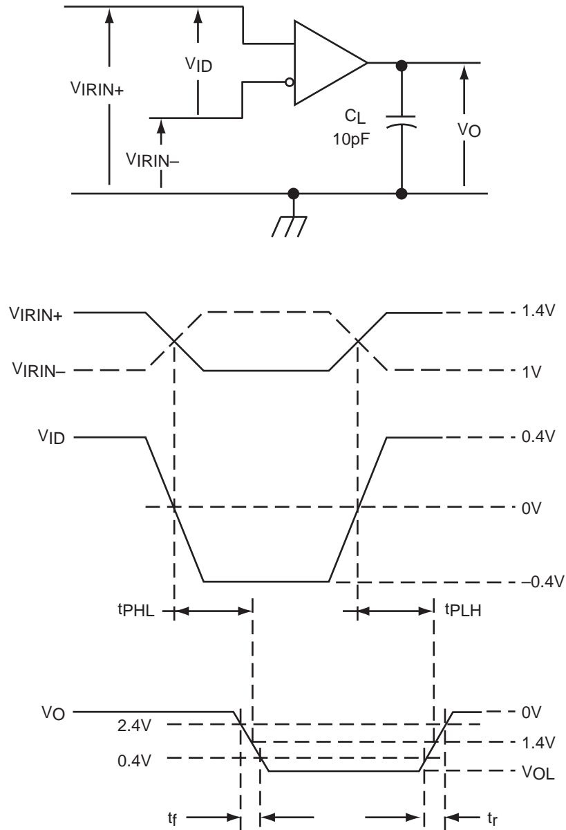
Figure 2. Timing Test Circuit and Waveforms
