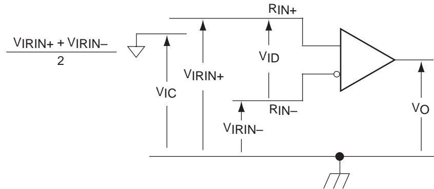
Figure 1. Voltage Definitions
