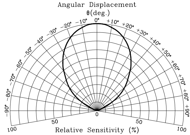
Sensitivity Diagram
