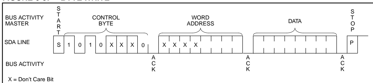
FIGURE 6-5: BYTE WRITE
