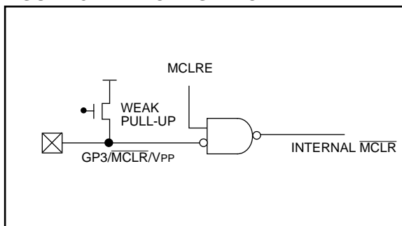
FIGURE 8-7: \overline{\text{MCLR}} SELECT
