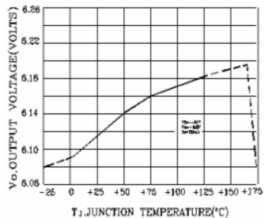
6 - OUTPUT VOLTAGE AS A OF JUNCTION TEMPERATURE
