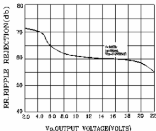
FIGURE 5 - RIPPLE REJECTION AS A FUNCTION FUNCTION OF OUTPUT VOLTAGES
