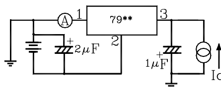
TEST CIRCUIT 3
