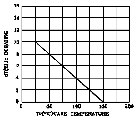
POWER DERATING
