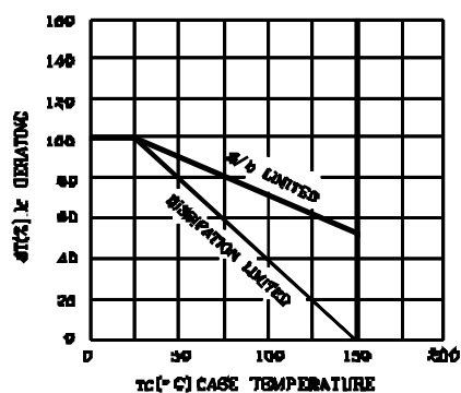
DERATING CURVE OF SAFE OPERATING AREAS
