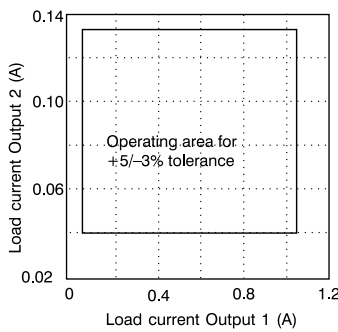
Cross regulation output 1 (+5V)
