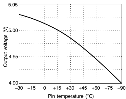
Temperature coefficient
